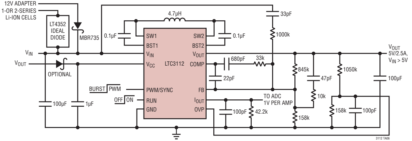
Adapter Plug-In
