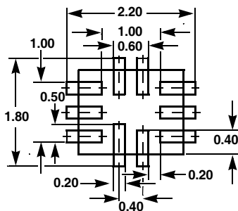
LAND PATTERN
