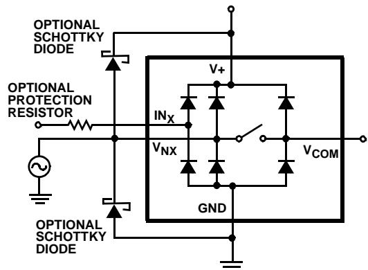
FIGURE 7. OVERVOLTAGE PROTECTION
