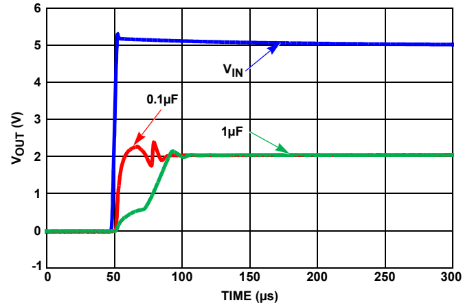
FIGURE 11. TURN-ON TIME
