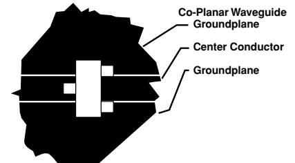
Figure 20. Circuit Layout.
