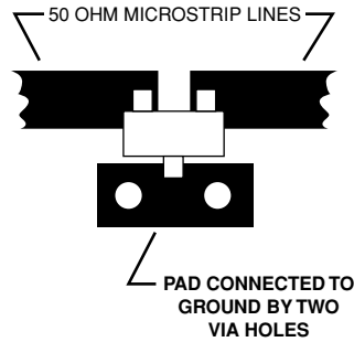
Figure 18. Circuit Layout.
