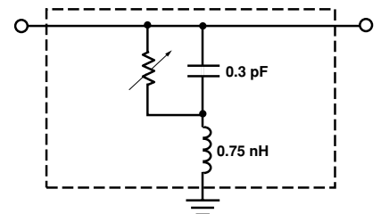
Figure 21. Equivalent Circuit.
