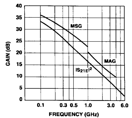
Figure 3. Insertion Power Gain, Maximum Available Gain and Maximum Stable Gain vs. Frequency. V_{CE} = 8\text{ V} , I_C = 35\text{ mA} .
