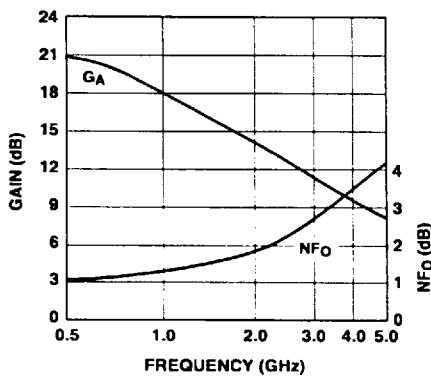
Figure 4. Noise Figure and Associated Gain vs. Frequency. V_{CE} = 8\text{ V} , I_C = 10\text{ mA} .
