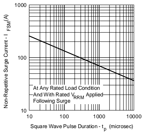
Fig. 7- Max. Non-Replicative Surge Current (Per Leg)
