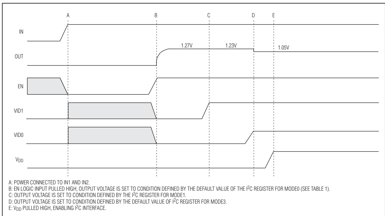
Figure 2. Power-Up Sequence
