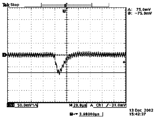
Vout=1.2V 50% to 100% load transients at 5V input and T_a=25^\circ C
