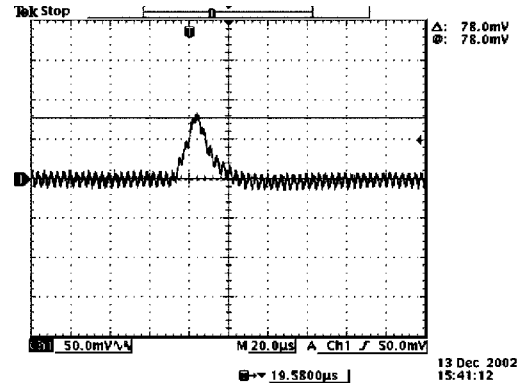
Vout=1.2V 100% to 50% load transients at 5V input and T_a=25^\circ C
