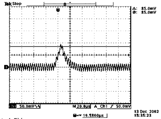
Vout=1.5V 100% to 50% load transients at 5V input and T_a=25^\circ C
