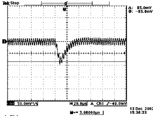
Vout=1.5V 50% to 100% load transients at 5V input and T_a=25^\circ C
