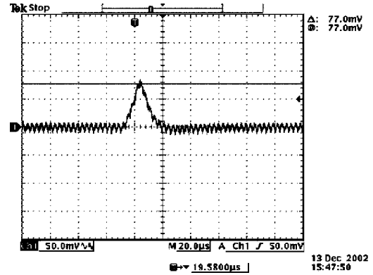
Vout=0.9V 100% to 50% load transients at 5V input and T_a=25^\circ C
