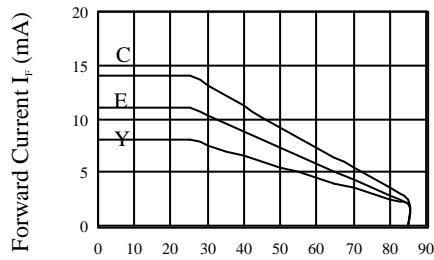
Ambient Temperature (°C) FIG.3 FORWARD CURRENT DERATING CURVE
