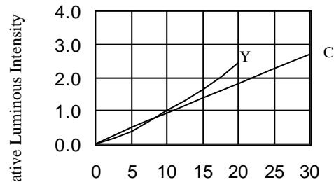
Forward Current I_F (mA) FIG.2 RELATIVE LUMINOUS INTENSITY VS. FORWARD CURRENT
