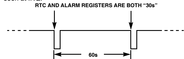
FIGURE 13. \overline{IRQ} WAVEFORM
