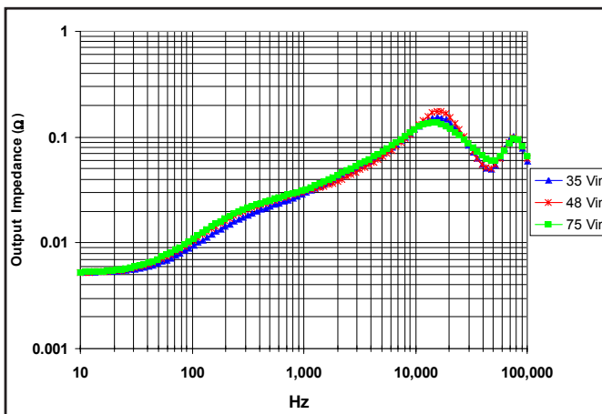
Figure 26: Output impedance ( Z_{out2} = V_{out2}/I_{out2} ) for minimum, nominal, and maximum input voltage at full rated power, for 5.0V output.
