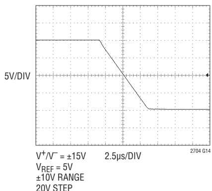
Negative Slew
