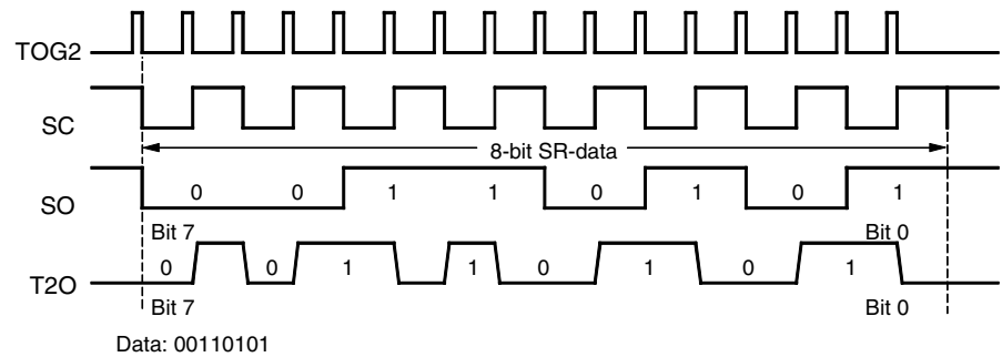
Figure 56. Manchester Modulation 1
