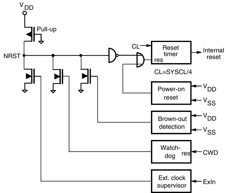
Figure 9. Reset Configuration
