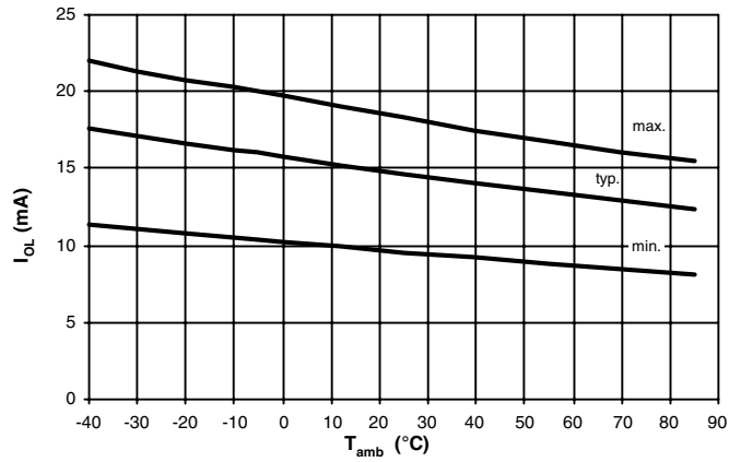
Figure 82. Output Low Current versus T_{\text{amb}} , V_{\text{DD}} = 6.5\text{ V} , V_{\text{OL}} = 0.2 \times V_{\text{DD}}
