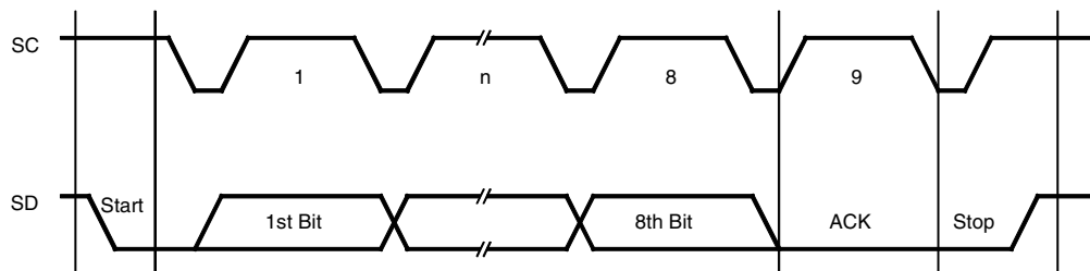
Figure 50. MCL Bus Protocol 2
