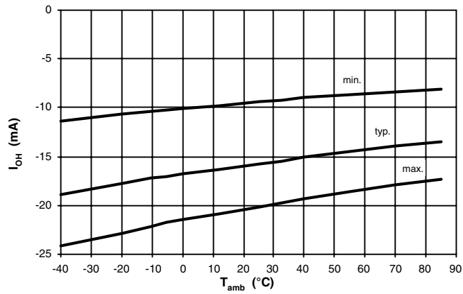
Figure 81. Output High Current versus T_{\text{amb}} = 25^{\circ}\text{C} , V_{\text{DD}} = 6.5\text{ V} , V_{\text{OH}} = 0.8 \times V_{\text{DD}}
