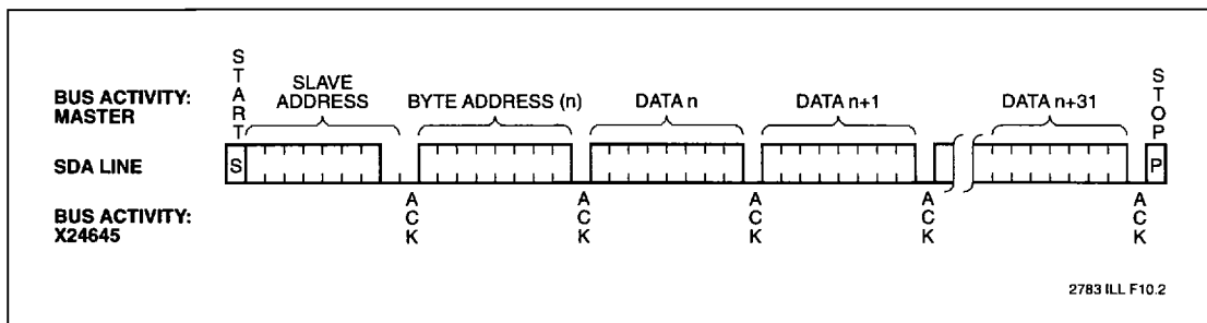
Figure 6. Page Write
