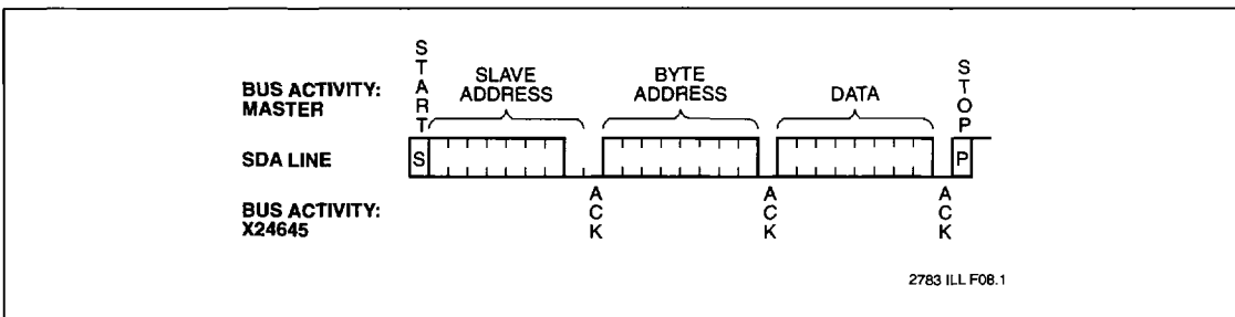
Figure 5. Byte Write
