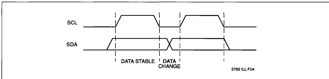
Figure 1. Data Validity
