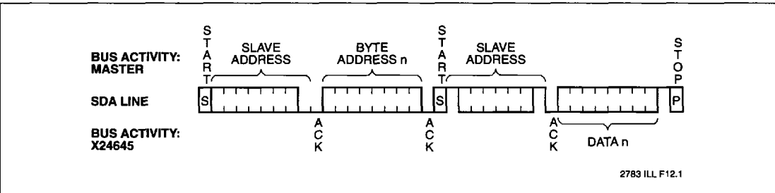
Figure 8. Random Read
