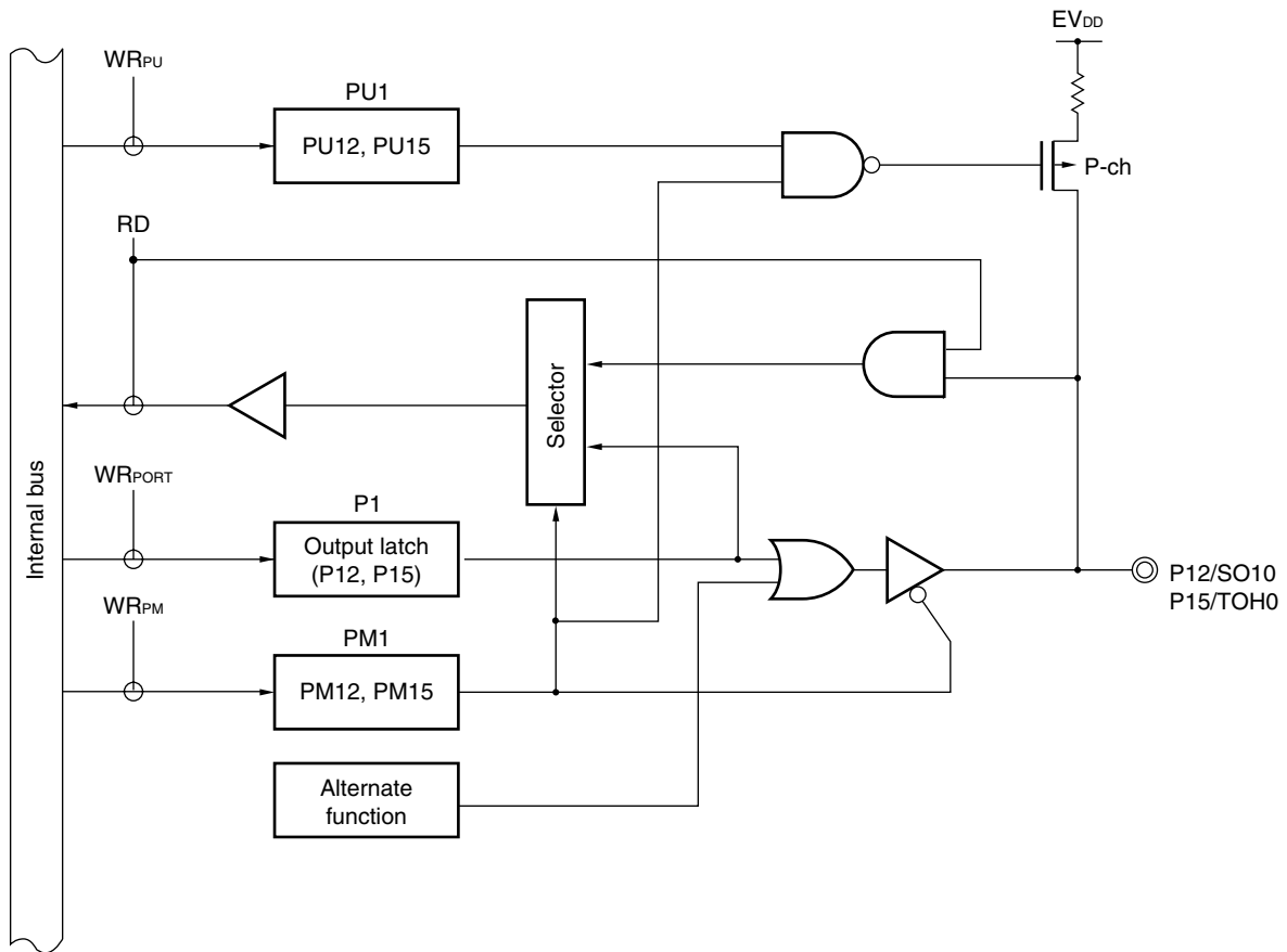
Figure 5-10. Block Diagram of P12 and P15
