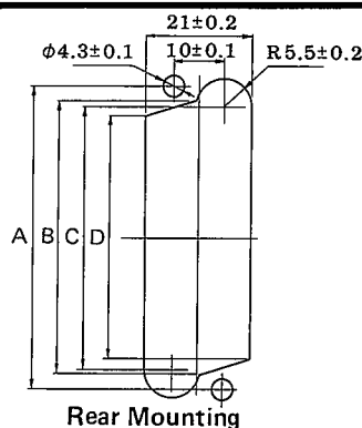
Rear Mounting
