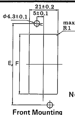
Front Mounting
