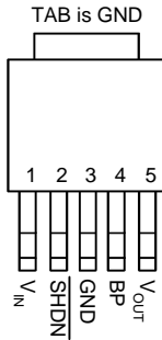
TO-252-5 (Top View)
