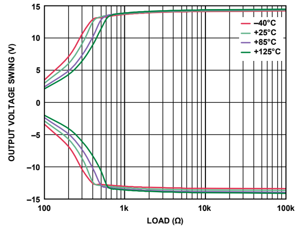
Figure 26. Output Voltage Swing vs. Load Resistance, V_S = \pm 15 V
