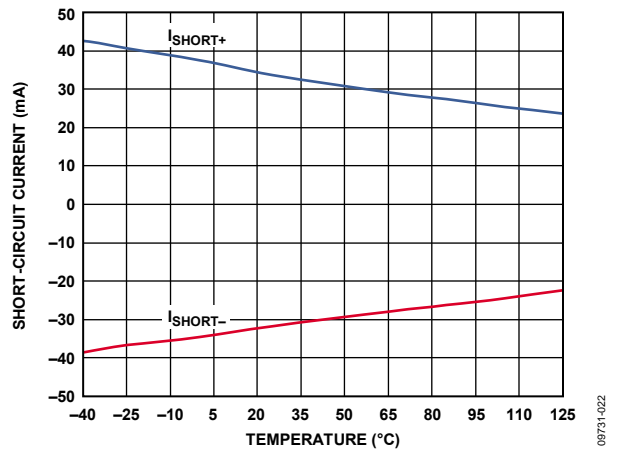
Figure 20. Short-Circuit Current vs. Temperature
