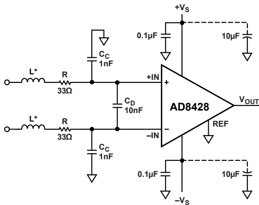
Figure 44. RFI Suppression
