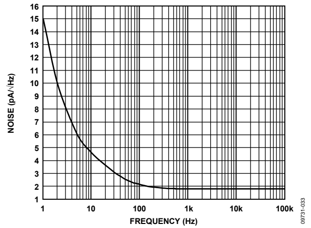
Figure 31. Current Noise Spectral Density vs. Frequency
