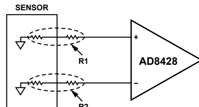
Figure 45. Source Resistance from Sensor and Protection Resistors
