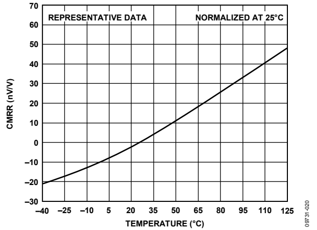
Figure 18. CMRR vs. Temperature, Normalized at 25°C
