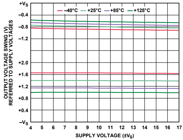
Figure 24. Output Voltage Swing vs. Supply Voltage, R_L = 10 k\Omega
