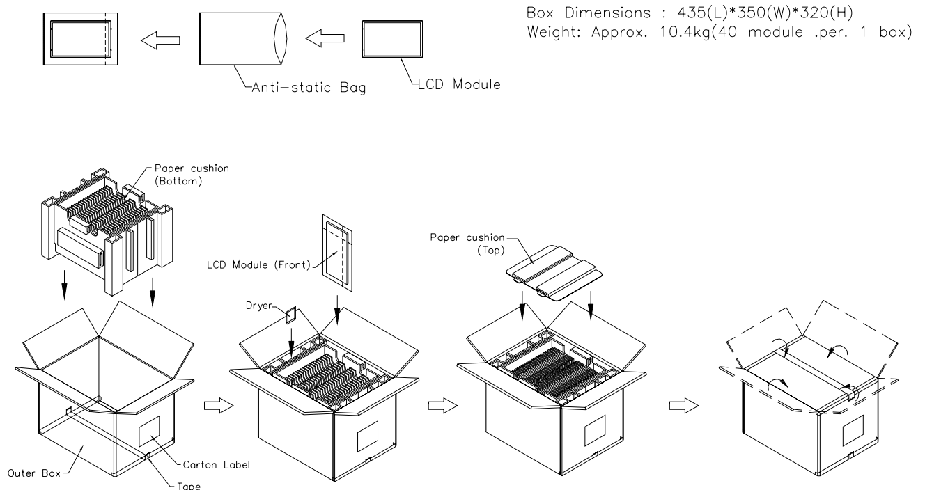
Figure. 10-1 Packing method
