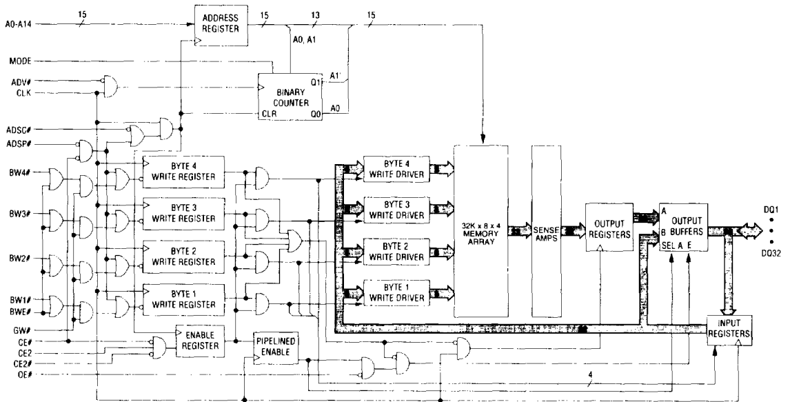
FUNCTIONAL BLOCK DIAGRAM 32K x 32
