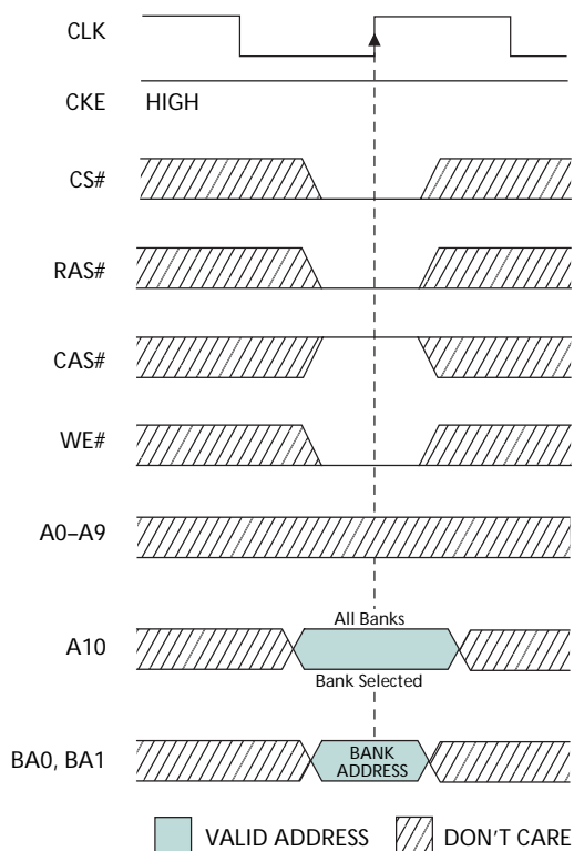
Figure 26: PRECHARGE Command
