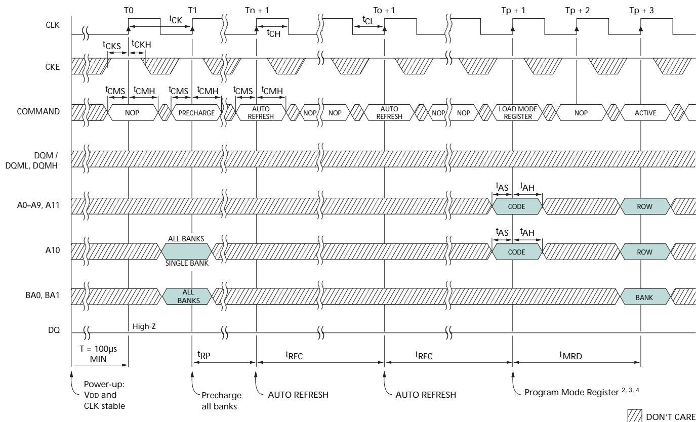
Figure 37: Initialize and Load Mode Register
