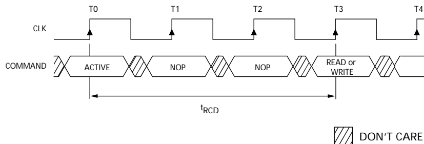
Figure 10: Example: Meeting t_{RCD} (MIN) When 2 < t_{RCD} (MIN)/t_{CK} \leq 3
