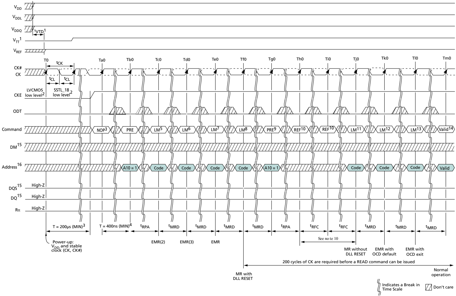
Figure 42: DDR2 Power-Up and Initialization
