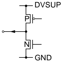
Fig. 4-11: Output Pins 6, 8, 9, and 10 (I2S_DA_OUT, ADR_DA, ADR_WS, ADR_CL)
