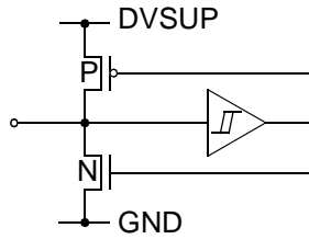
Fig. 4-15: Input/Output Pins 4, 5, 77, and 78 (I2S_CL, I2S_WS, D_CTR_I/O_1, D_CTR_I/O_0)
