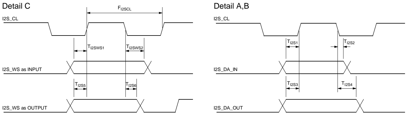
Fig. 4–26: I 2 S bus timing diagram
