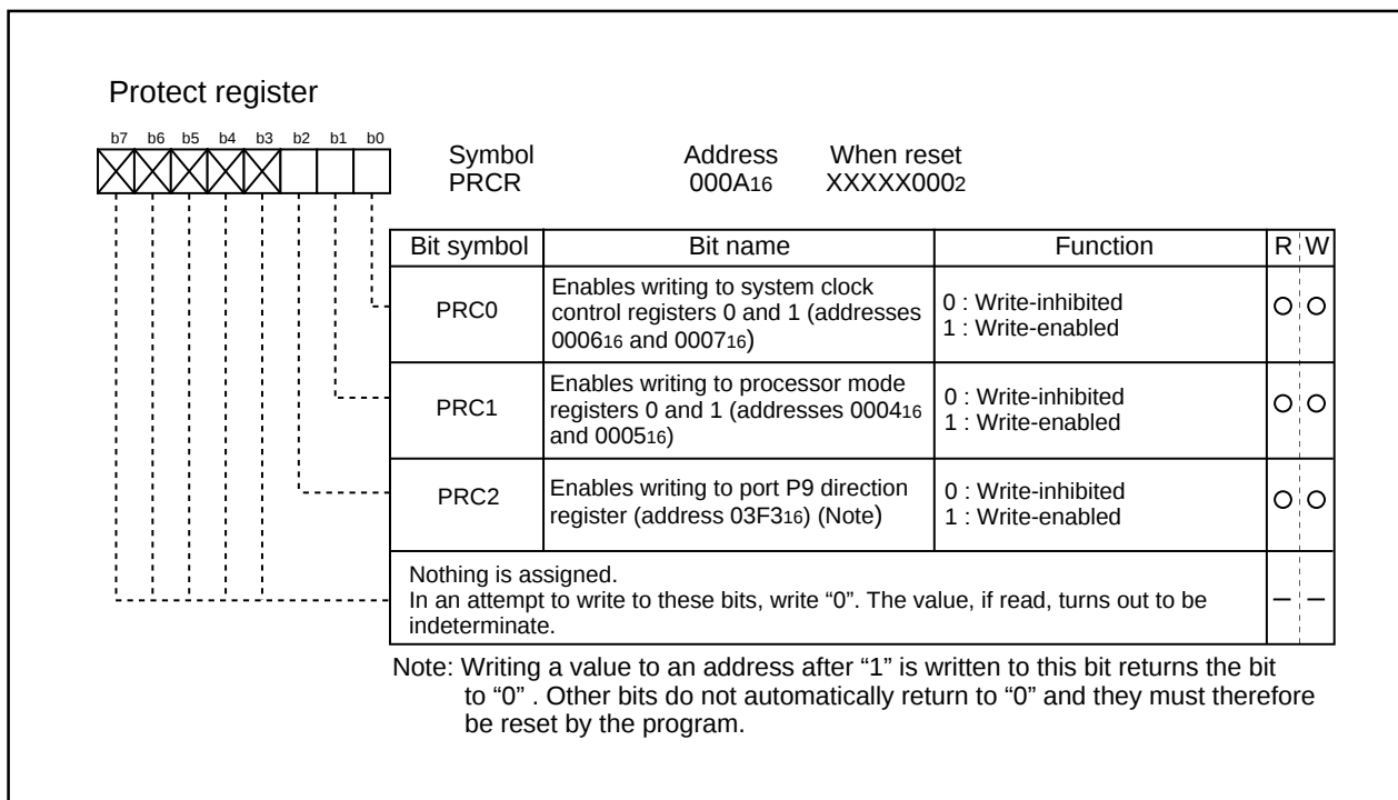
Figure 1.10.6. Protect register
