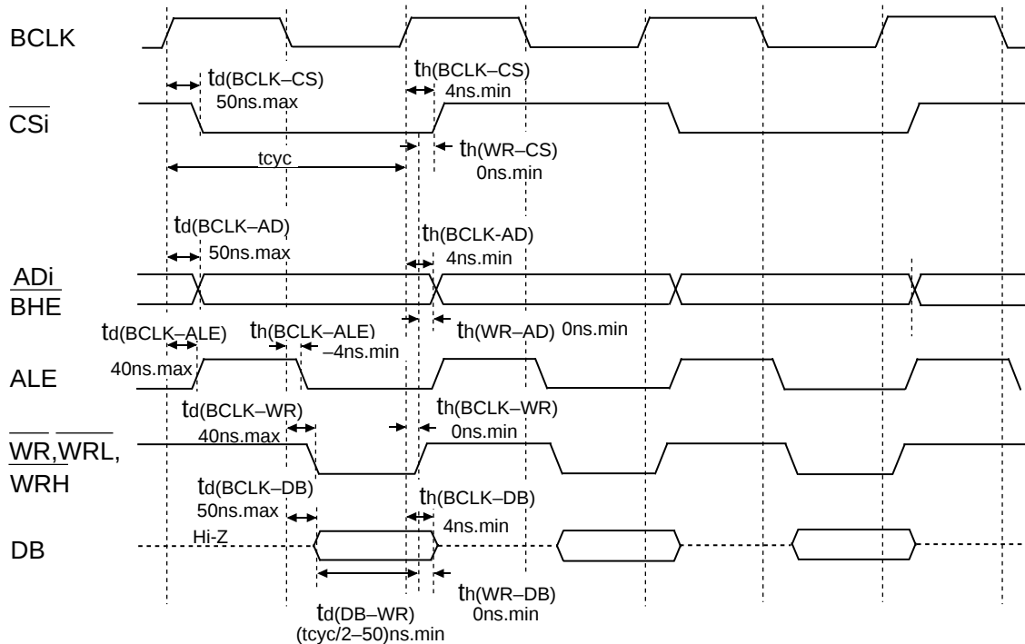
Figure 1.26.4. Timing diagram (3)
