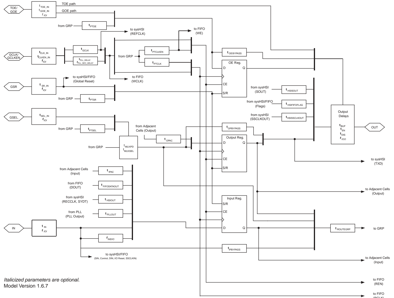
Figure 17. ispGDX2 Timing Model Diagram (I/O Cell)
