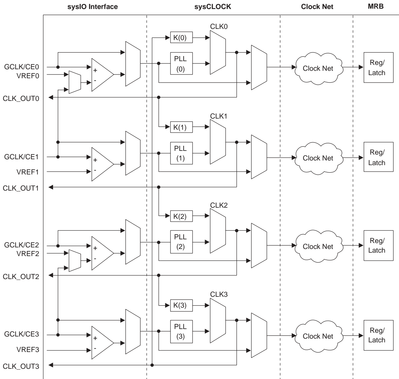
Figure 8. ispGDX2-256 CLOCK Network
