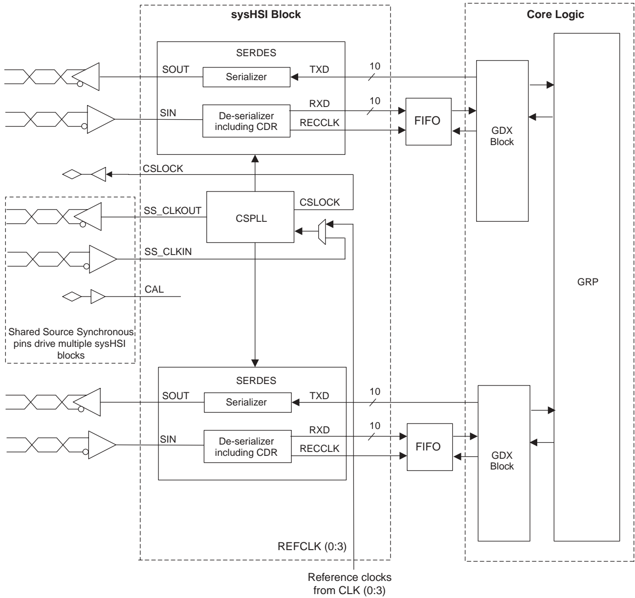
Figure 13. sysHSI Block with SERDES and FIFO
