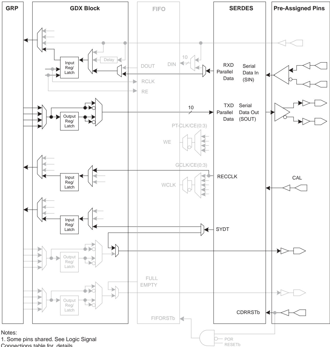
Figure 14. Operation in SERDES Only Mode 1,2
