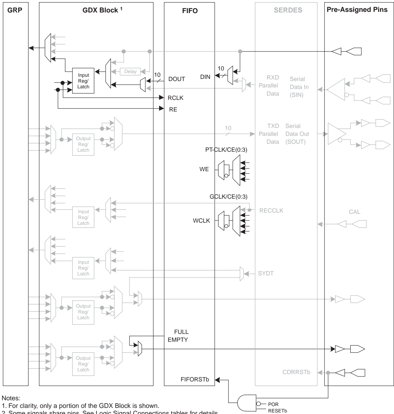
Figure 12. Operation in FIFO Mode 2
