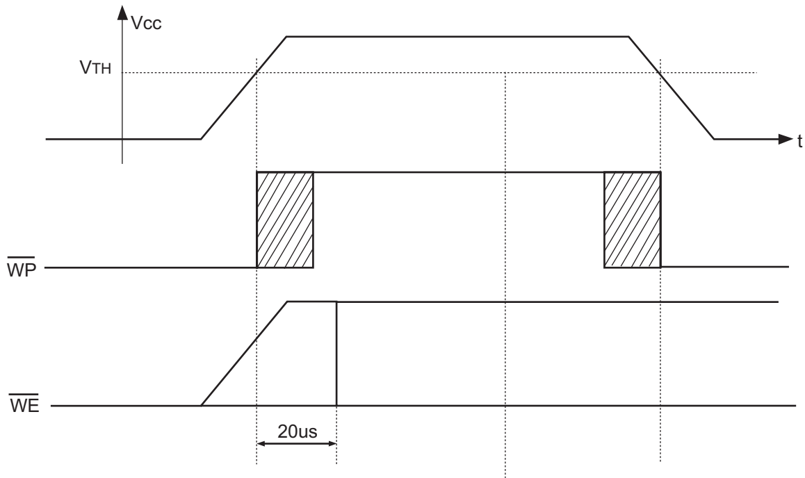
Figure 32: Power On and Data Protection Timing
