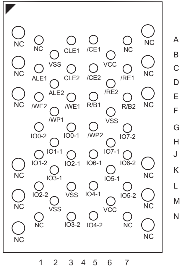
Figure 4. 52-ULGA Contactations, x8 Device, Dual interface (Top view through package)
