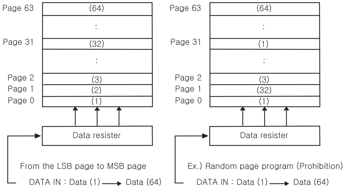
Figure 35 : page programming within a block
