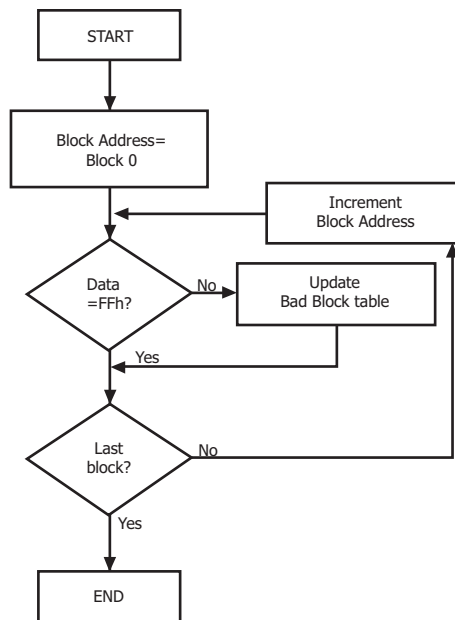
Figure 36: Bad Block Management Flowchart
