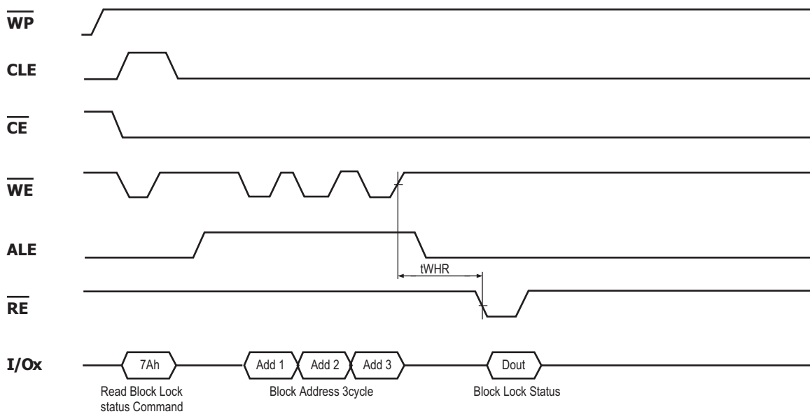
Figure 29: Lock Status Read Timing
