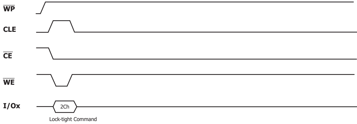
Figure 28: Lock Tight Command
