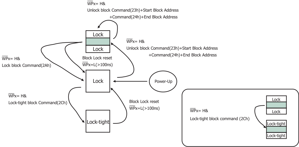
Figure 34: Lock/Unlock FSM Flow Cart
