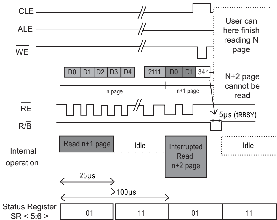
Figure 23: exit from cache read in 5us when device internally is reading
