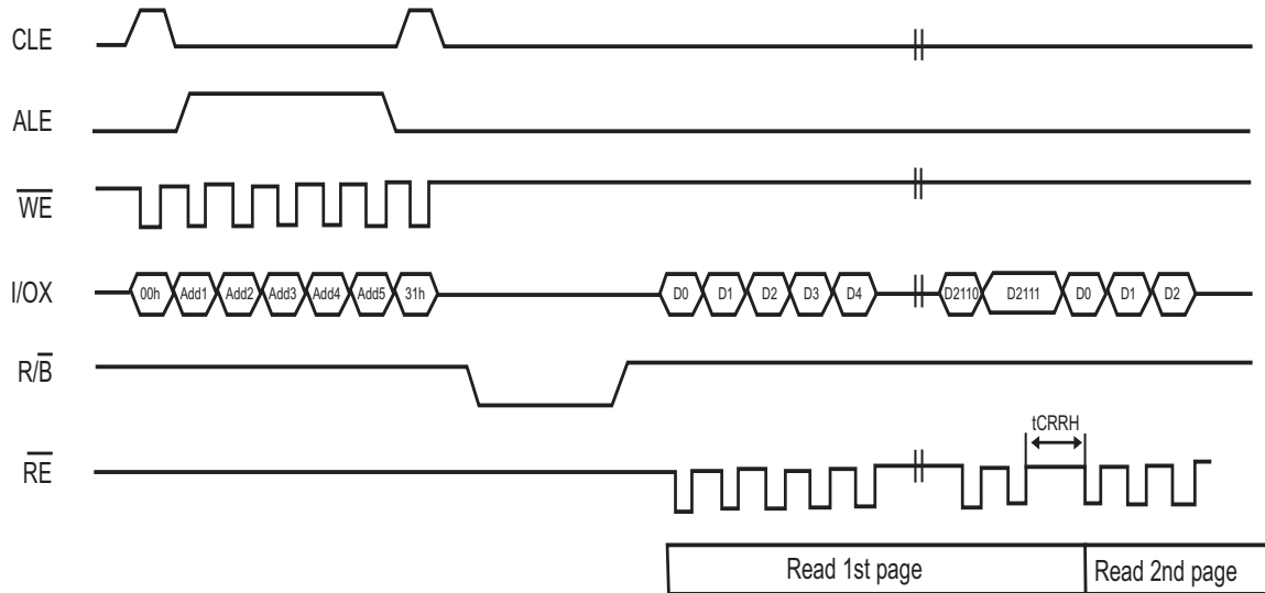
Figure 18: Cache Read RE# high
