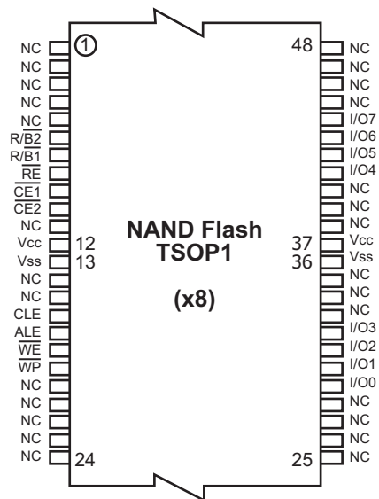
Figure 3. 48TSOP1 Contactions, x8 Device (2CE)
