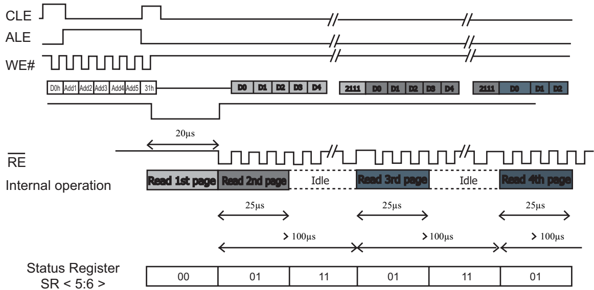
Figure 22: start address at page start :after 1st latency uninterrupted data flow
