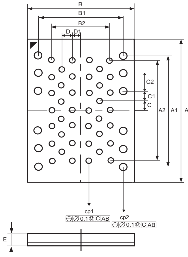
Figure 42. 52-ULGA, 12 x 17mm, Package Outline (Top view through package)
