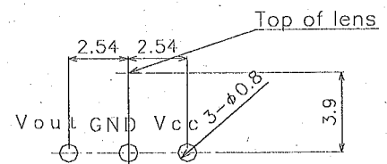
Example of mounting drawing from solder side (Reference)
