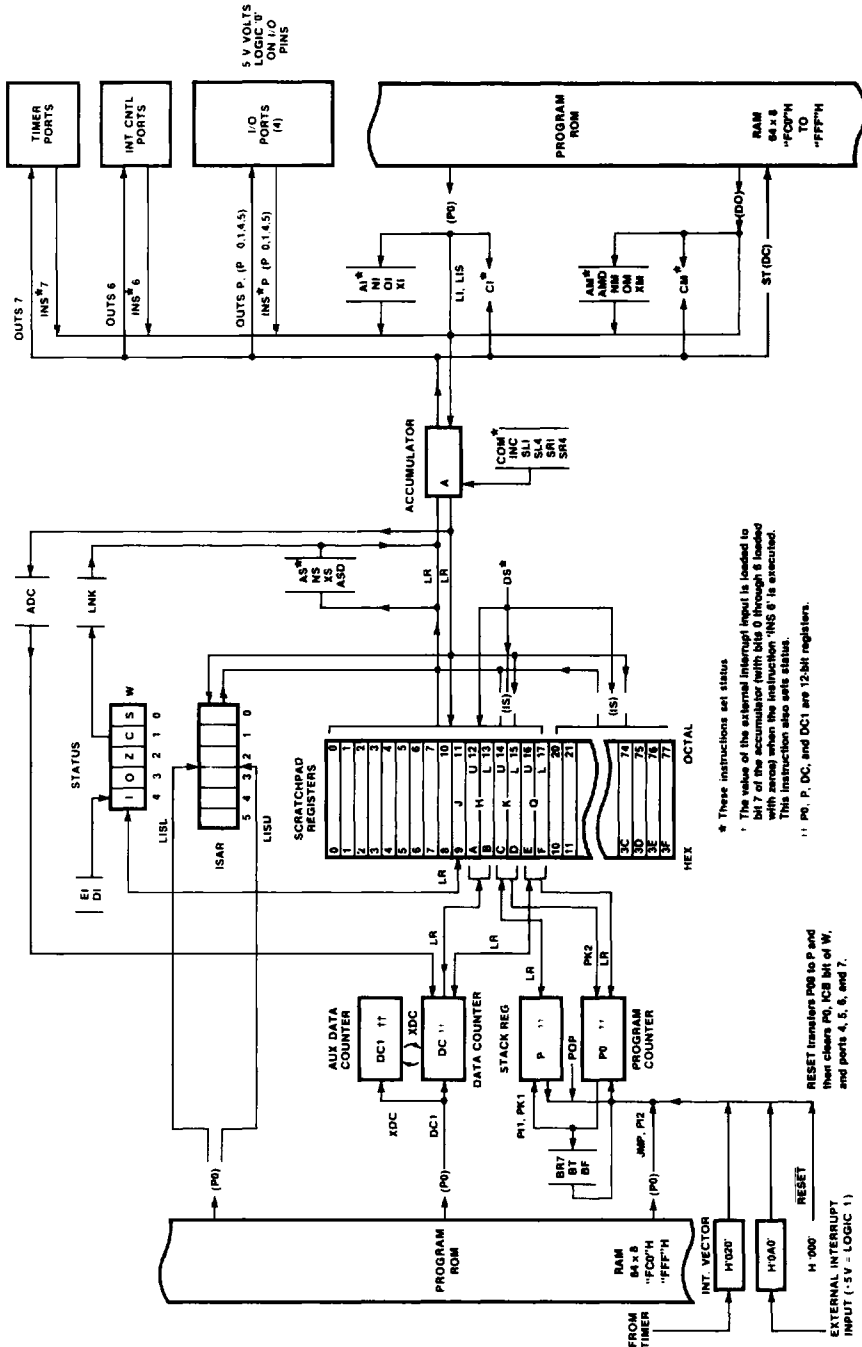
Fig. 9 Programming Model
