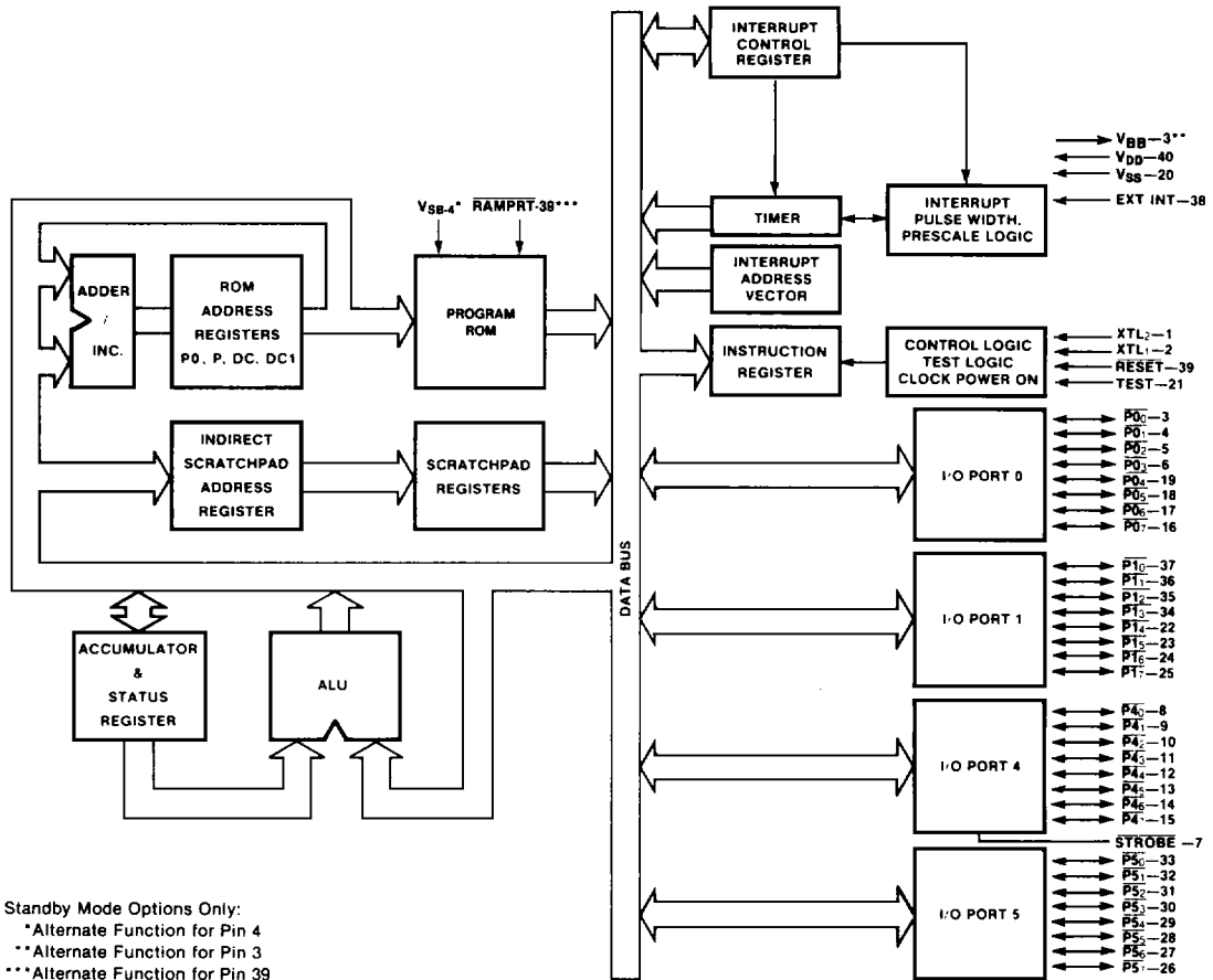
Fig. 2 F3872 Block Diagram
