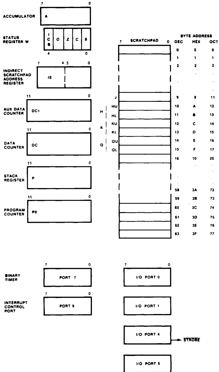
Fig. 8 Programmable Registers and Ports
