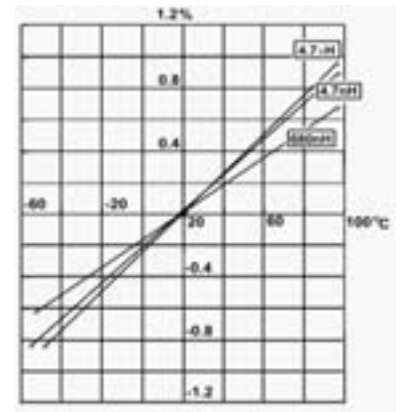
Temperature Characteristic
