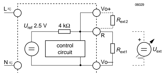
Fig. 19 Output voltage control for single output units, -0503- types and double output units fitted with option R by means of the R input.
