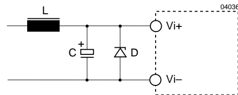
Fig. 8 Example for external circuitry to comply with IEC/EN 61000-4-5 or ETR 283 (19Pfl1); the suppressor diode D is only necessary for 20 IMX 15 types.
