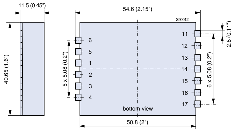
Fig. 27 Surface mount version with PCB lid (option L)
