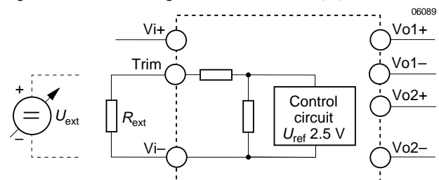
Fig. 20 Output voltage control for double output units by means of the Trim input.
