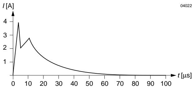
Fig. 6 Typical inrush current at U_{i\text{ nom}} , P_{o\text{ nom}} versus time (40 IMX 15). Source impedance according to ETS 300132-2 at U_{i\text{ nom}} .
