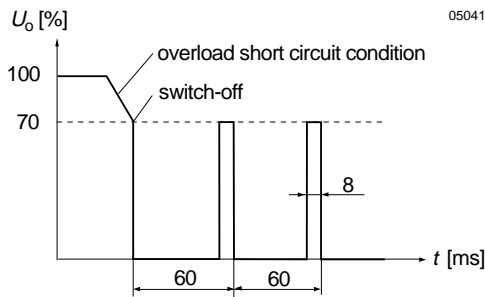
Fig. 15 Overload switch off (hiccup mode), typical values.
