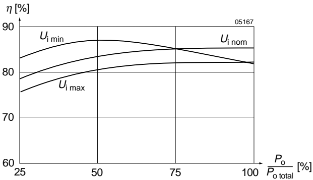
Fig. 14 Efficiency versus input voltage and load. Typical values 40 IMX 15-12-12-7
