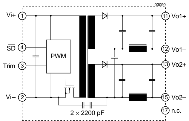
Fig. 4 Block diagram, double output types, standard pinout.
