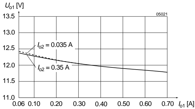
Fig. 13 Cross load regulation U_{o1} versus I_{o1} (typ) for various I_{o2} ( 2 \times 12 V).
