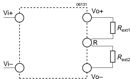
Fig. 18 Output voltage control for single output units synchronous rectification.
