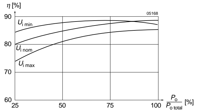
Fig. 17 Efficiency versus input voltage and load. Typical values 110 IMY 15-12-12-7
