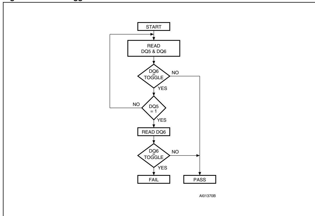
Figure 48. Data toggle flowchart
