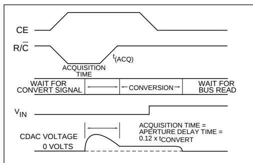
Figure 1. Sample-and-Hold Function
