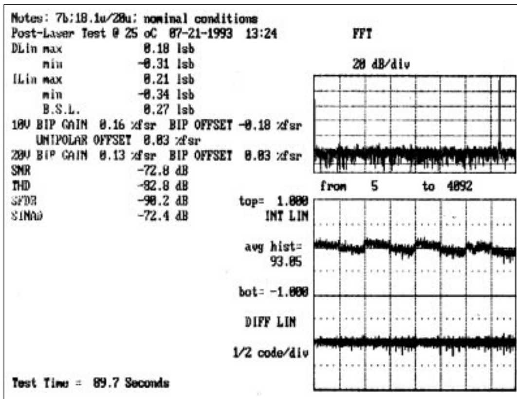
Figure 10. Typical FFT at Nyquist Sampling Rates
