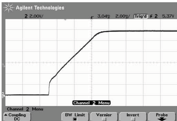
Figure 12. Enable Start-up (Vin=48V Iout=30A)
