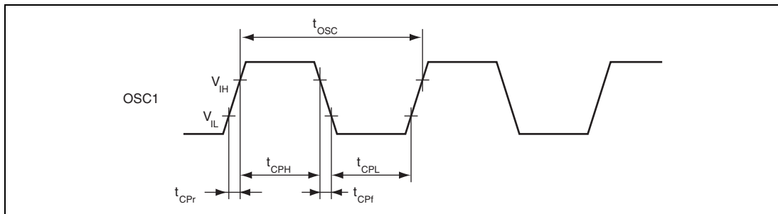
Figure 23.1 System Clock Input Timing
