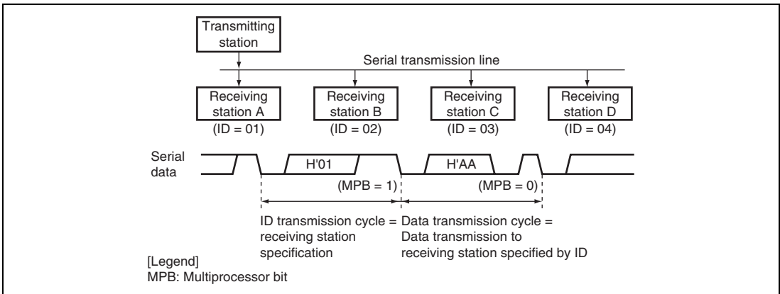
Figure 17.15 Example of Inter-Processor Communication Using Multiprocessor Format (Transmission of Data H'AA to Receiving Station A)
