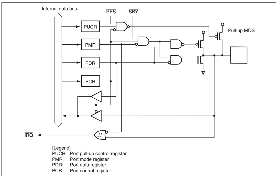
Figure B.2 Port 1 Block Diagram (P14, P16)
