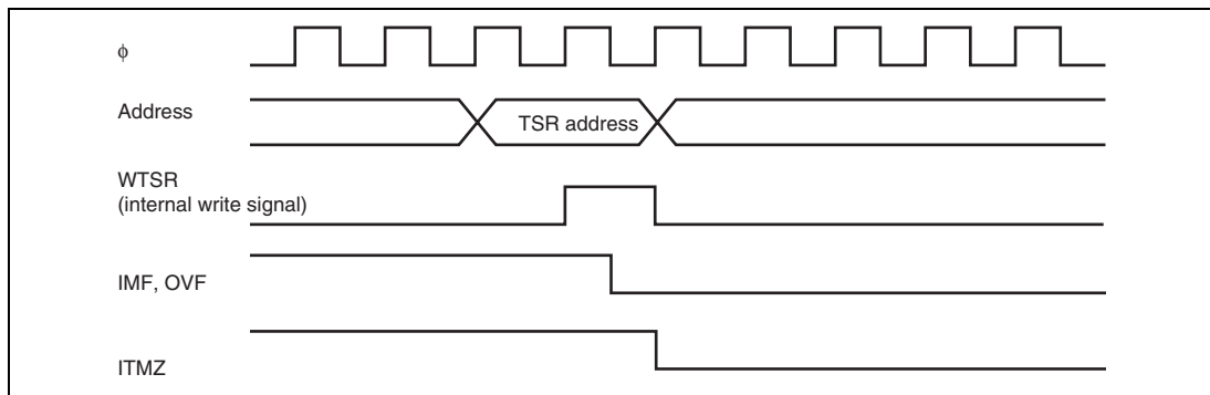
Figure 14.51 Status Flag Clearing Timing
