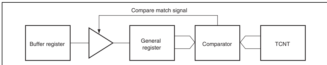
Figure 14.35 Compare Match Buffer Operation
