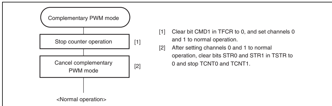
Figure 14.30 Canceling Procedure of Complementary PWM Mode
