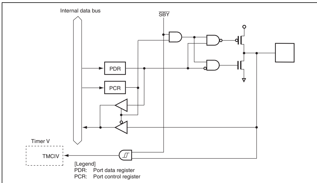
Figure B.18 Port 7 Block Diagram (P75)
