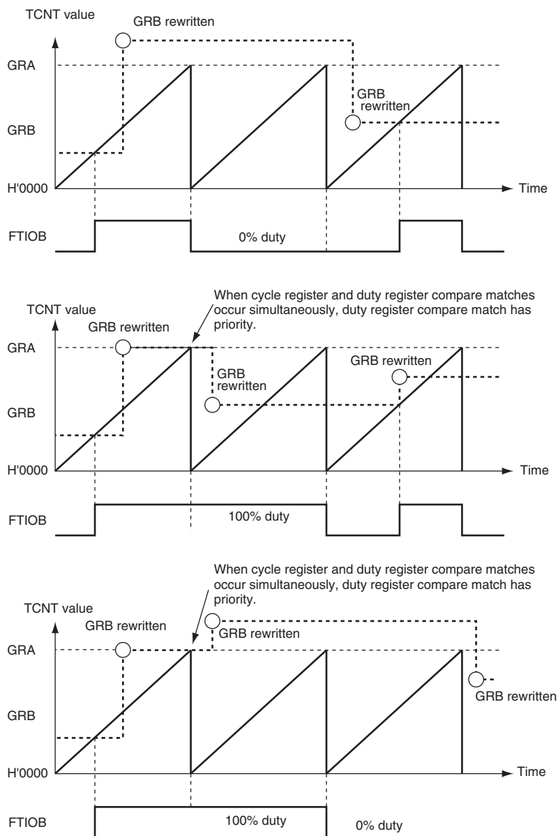
Figure 14.25 Example of PWM Mode Operation (4)
