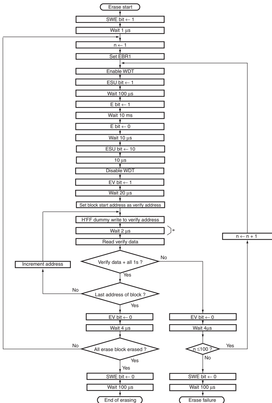
Figure 7.4 Erase/Erase-Verify Flowchart
