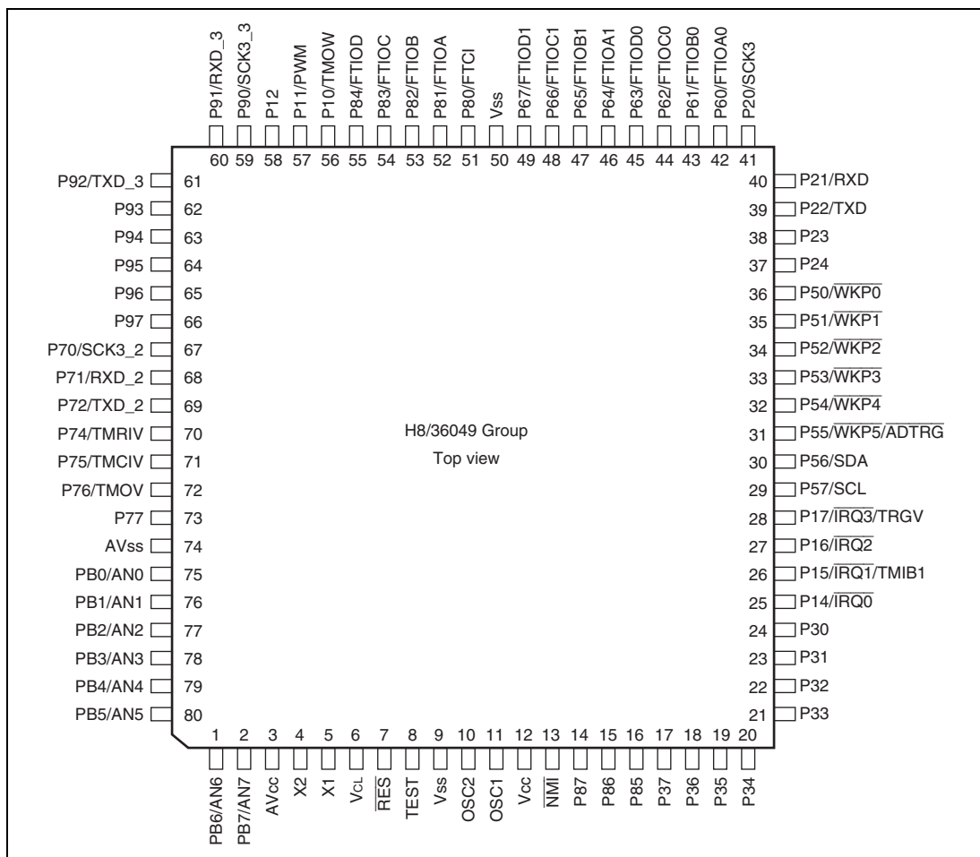
Figure 1.2 Pin Arrangements (FP-80A)
