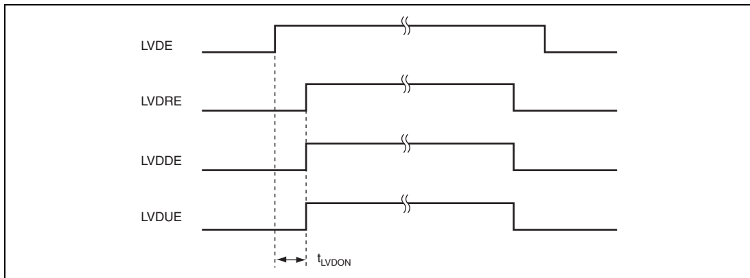
Figure 20.5 Timing for Operation/Release of Low-Voltage Detection Circuit
