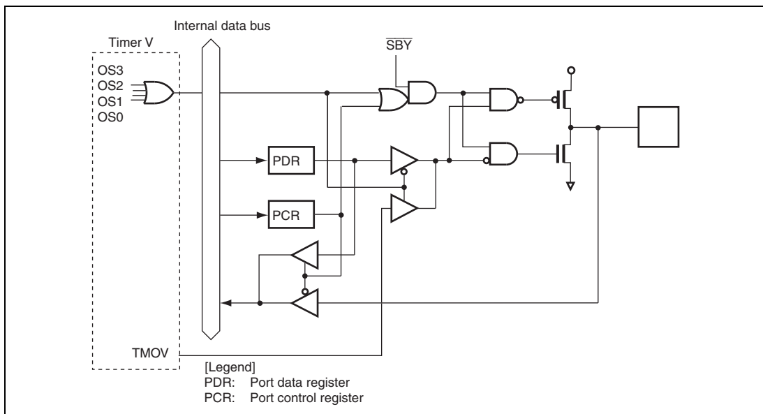
Figure B.17 Port 7 Block Diagram (P76)
