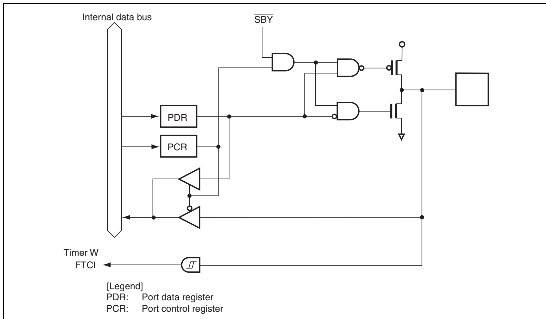
Figure B.25 Port8 Block Diagram (P80)
