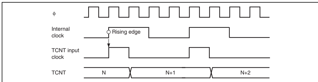
Figure 13.14 Count Timing for Internal Clock Source
