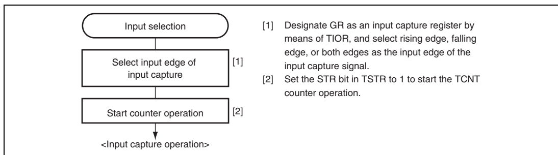
Figure 14.16 Example of Input Capture Operation Setting Procedure
