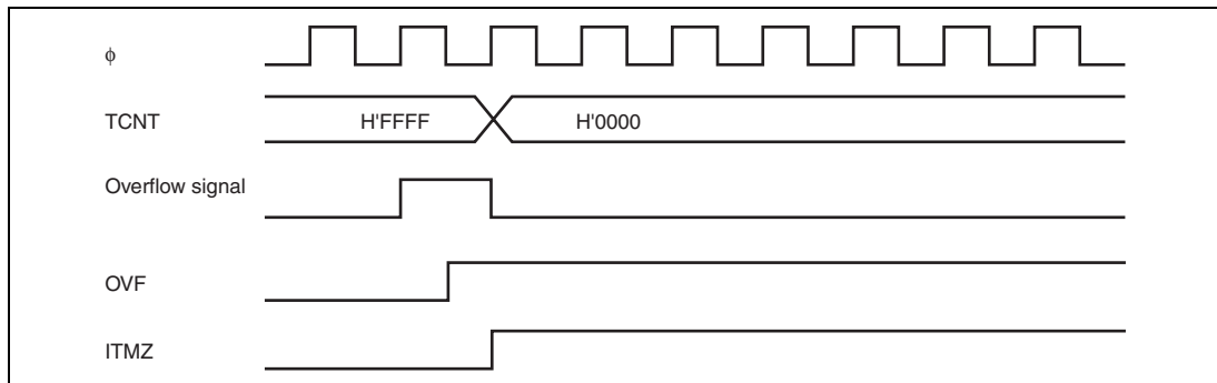
Figure 14.50 OVF Flag Set Timing
