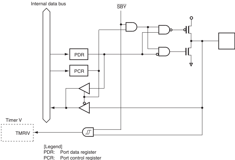
Figure B.19 Port 7 Block Diagram (P74)
