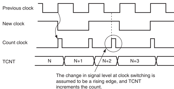
Figure 13.25 Internal Clock Switching and TCNT Operation
