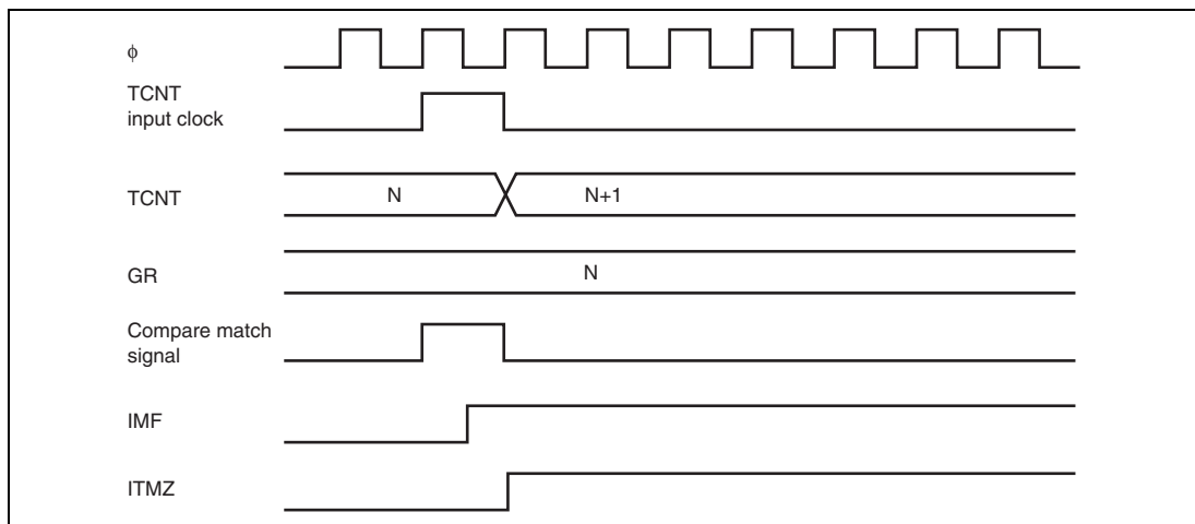
Figure 14.48 IMF Flag Set Timing when Compare Match Occurs
