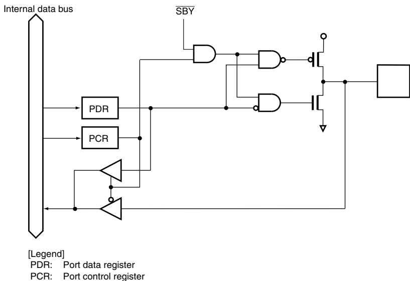
Figure B.26 Port 9 Block Diagram (P97 to P93)
