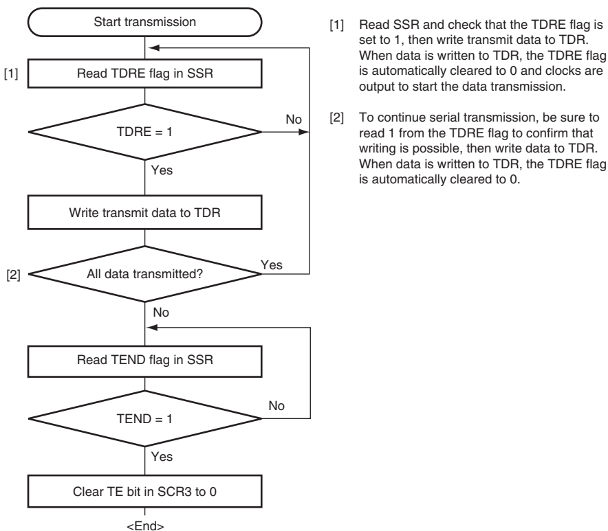
Figure 17.11 Sample Serial Transmission Flowchart (Clocked Synchronous Mode)
