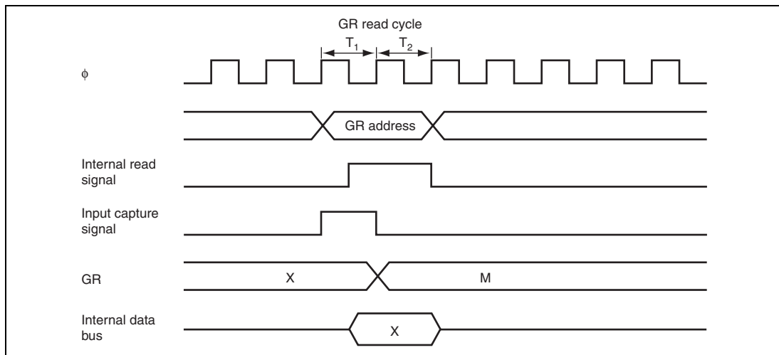
Figure 14.56 Contention between GR Read and Input Capture
