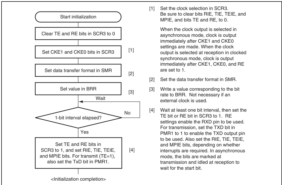
Figure 17.4 Sample SCI3 Initialization Flowchart
