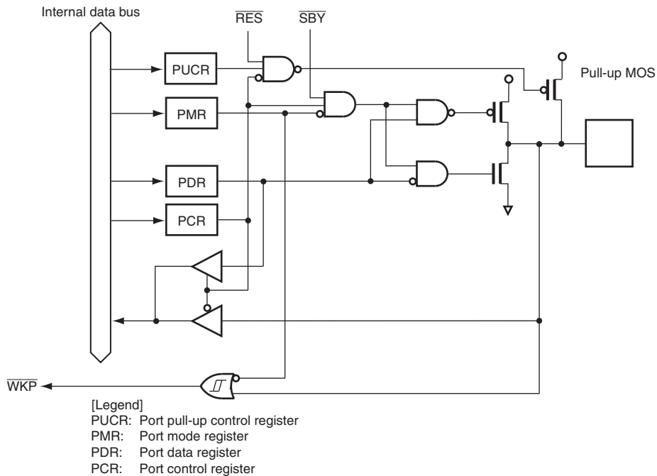
Figure B.14 Port 5 Block Diagram (P54 to P50)
