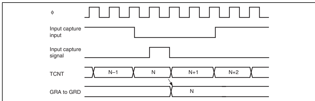
Figure 13.17 Input Capture Input Signal Timing
