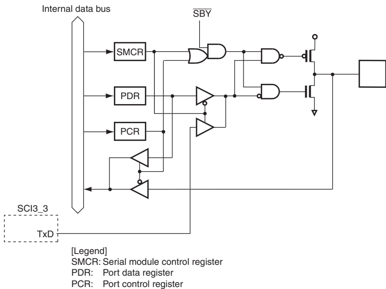
Figure B.27 Port 9 Block Diagram (P92)
