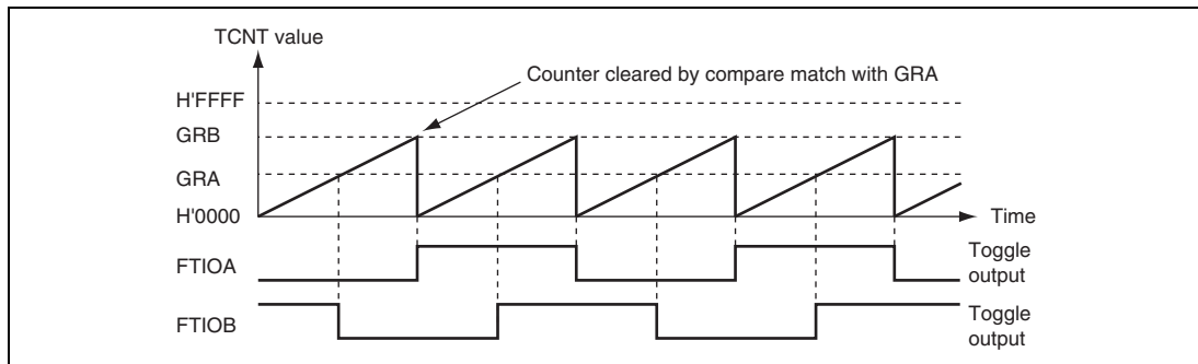
Figure 13.6 Toggle Output Example (TOA = 0, TOB = 1)
