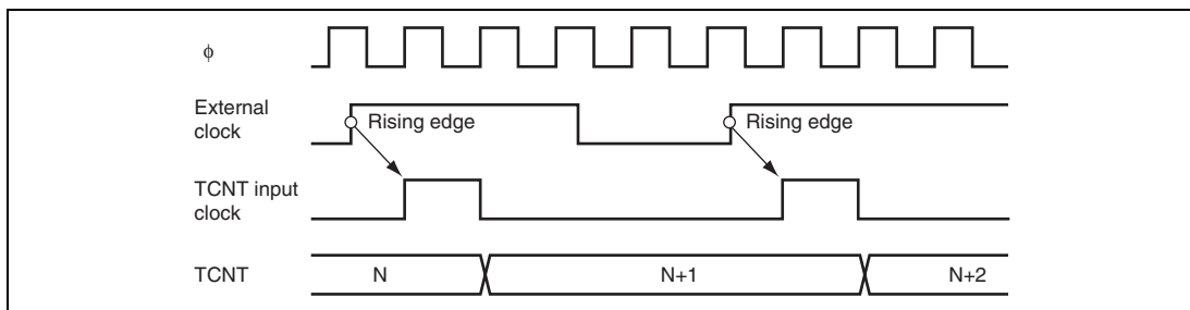
Figure 13.15 Count Timing for External Clock Source
