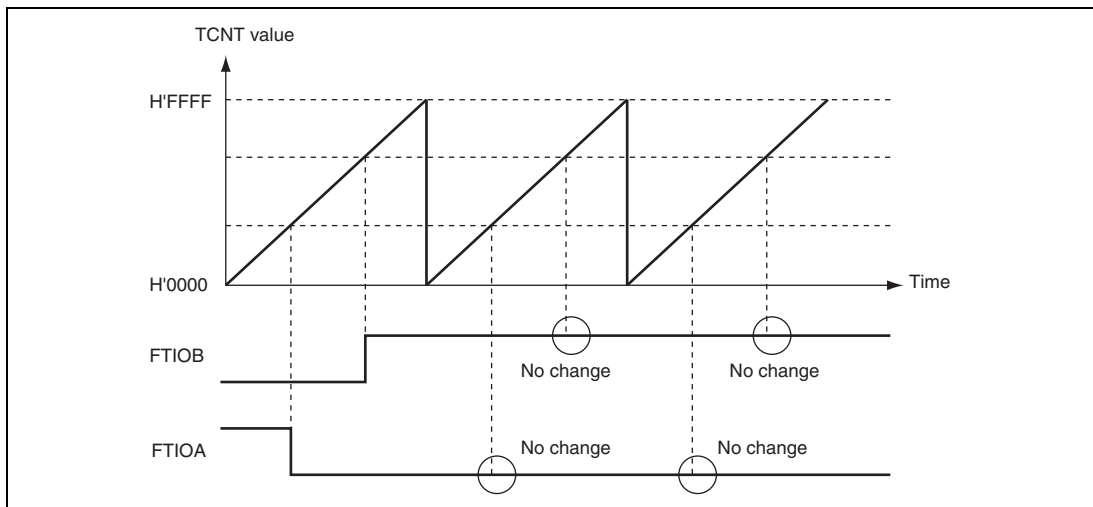
Figure 14.13 Example of 0 Output/1 Output Operation
