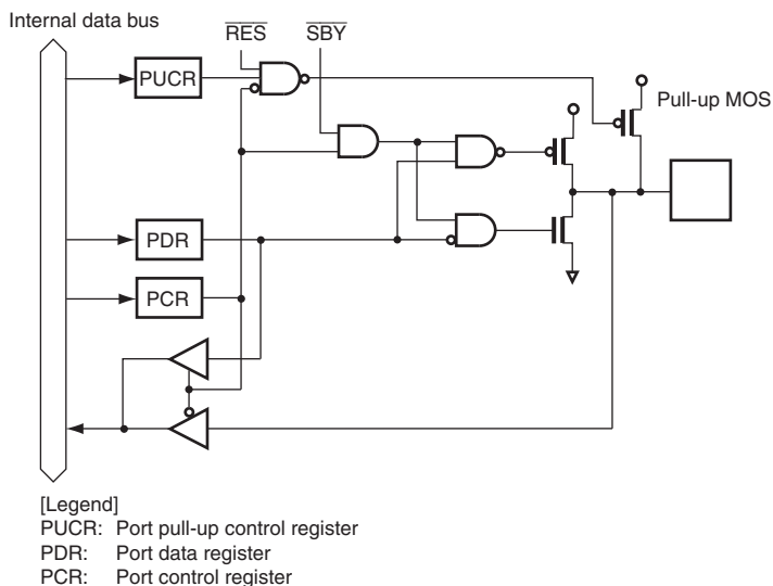
Figure B.4 Port 1 Block Diagram (P12)
