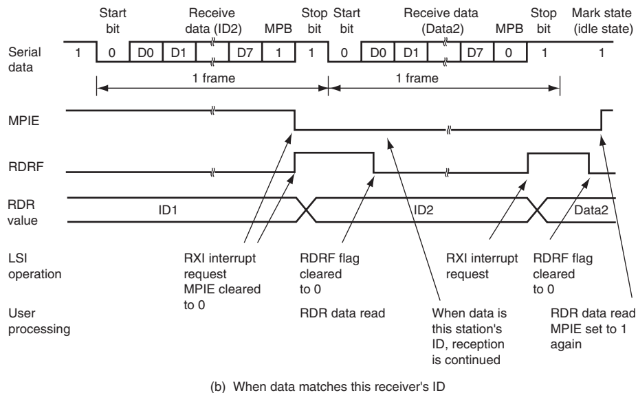
Figure 17.18 Example of SCI3 Reception Using Multiprocessor Format (Example with 8-Bit Data, Multiprocessor Bit, One Stop Bit)
