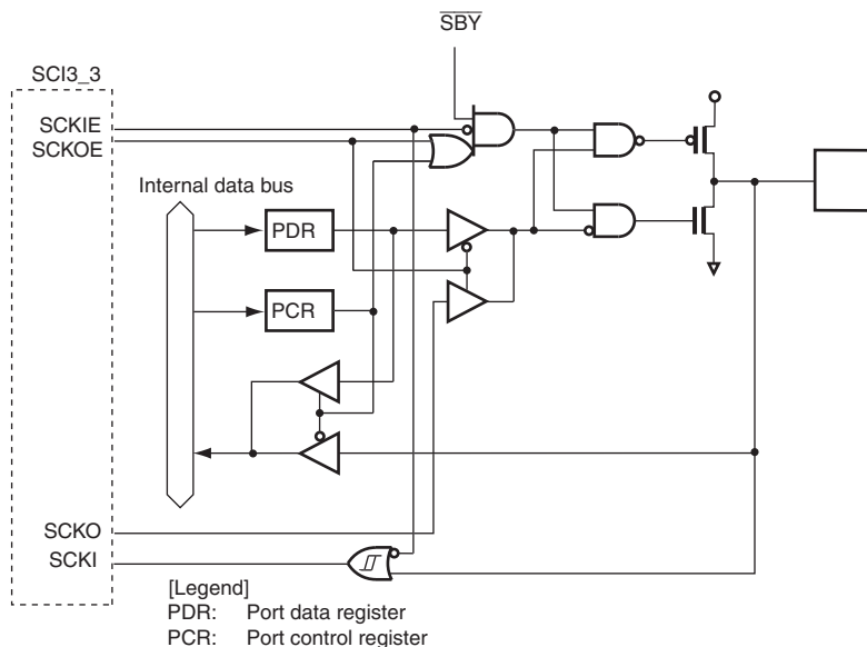
Figure B.29 Port 9 Block Diagram (P90)
