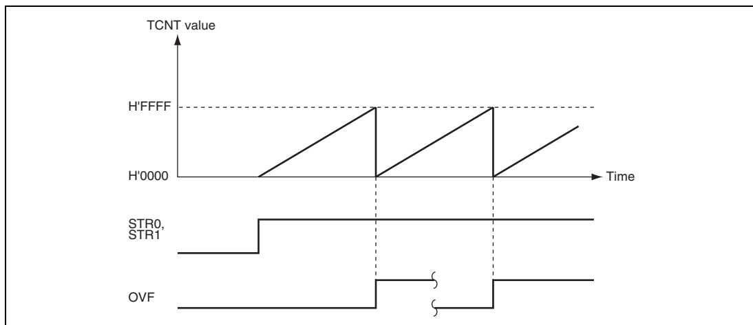
Figure 14.8 Free-Running Counter Operation
