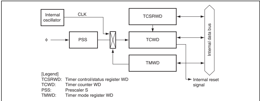
Figure 15.1 Block Diagram of Watchdog Timer
