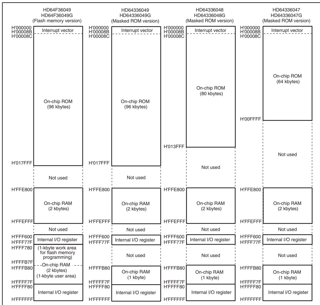
Figure 2.1 Memory Map
