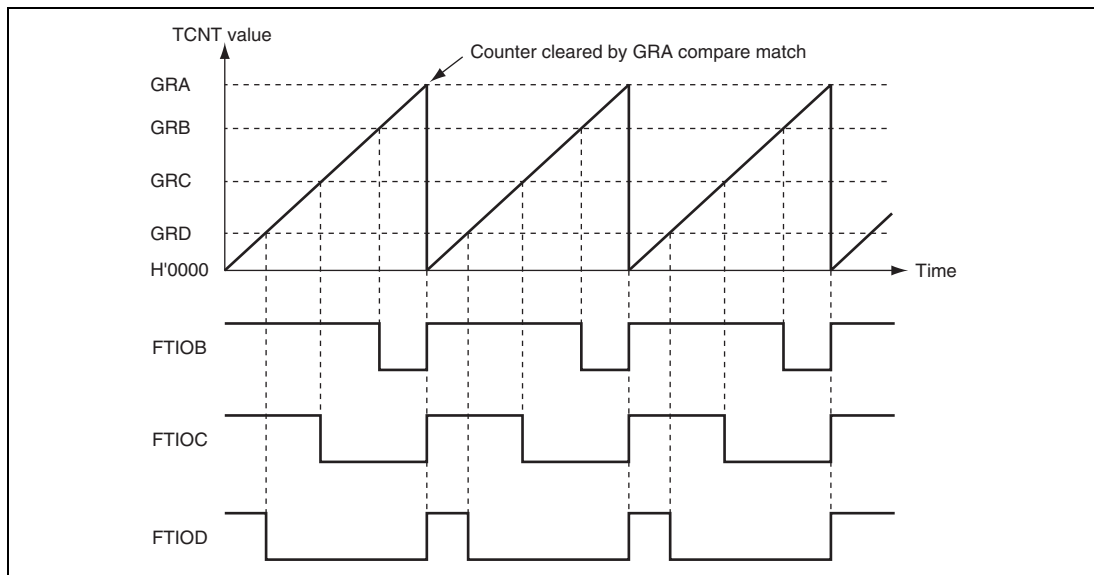
Figure 14.22 Example of PWM Mode Operation (1)
