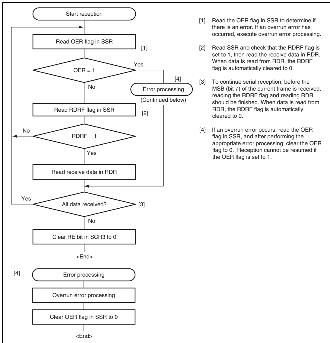
Figure 17.13 Sample Serial Reception Flowchart (Clocked Synchronous Mode)
