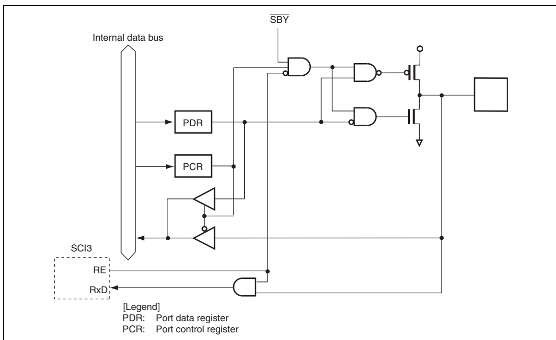
Figure B.9 Port 2 Block Diagram (P21)
