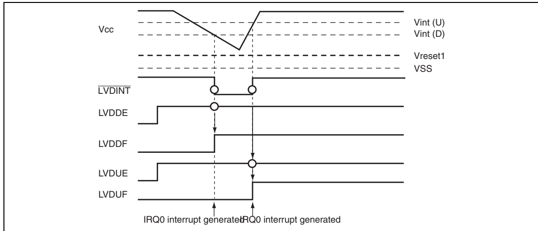
Figure 20.4 Operational Timing of LVDR Circuit
