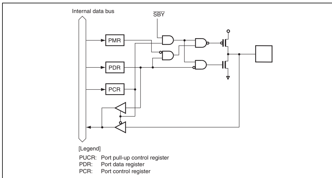
Figure B.7 Port 2 Block Diagram (P24, P23)
