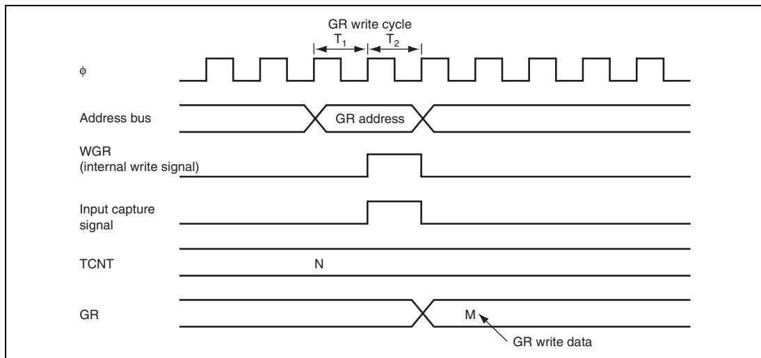
Figure 14.58 Contention between GR Write and Input Capture
