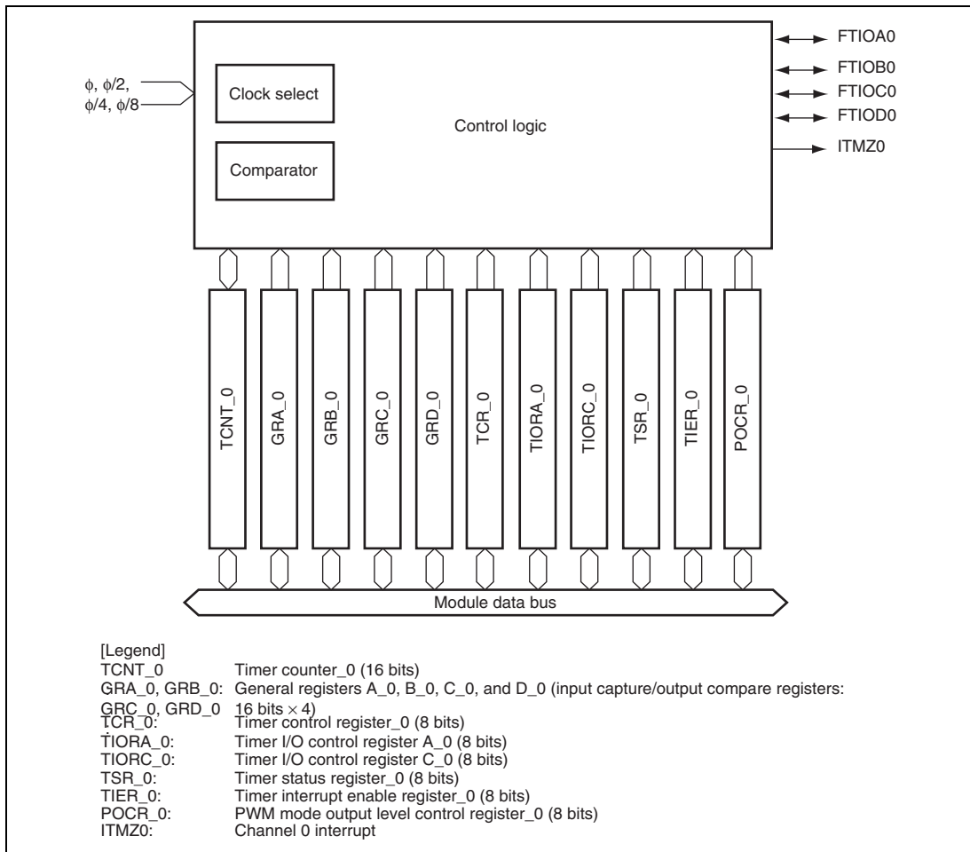
Figure 14.2 Timer Z (Channel 0) Block Diagram
