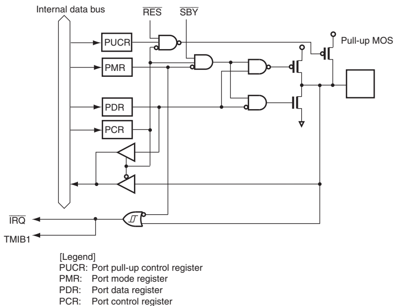
Figure B.3 Port 1 Block Diagram (P15)
