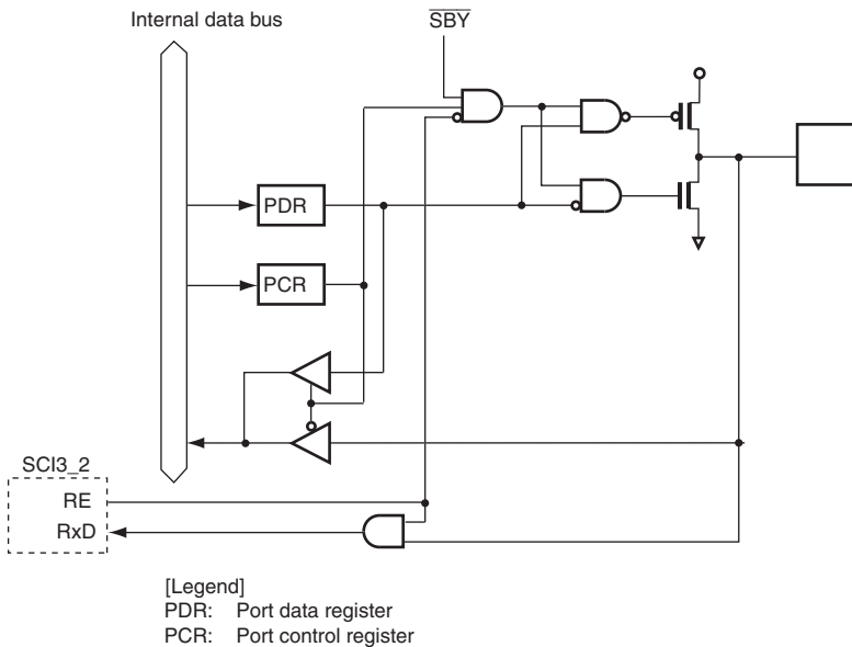
Figure B.21 Port 7 Block Diagram (P71)
