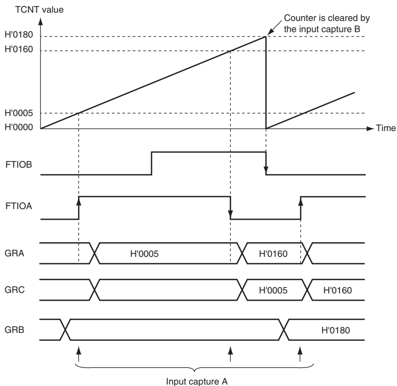
Figure 14.40 Example of Buffer Operation (2) (Buffer Operation for Input Capture Register)
