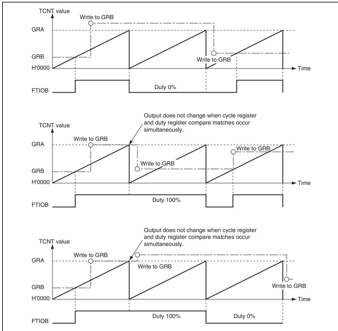
Figure 13.12 PWM Mode Example (TOB = 0, TOC = 0, TOD = 0: Initial Output Values are Set to 0)
