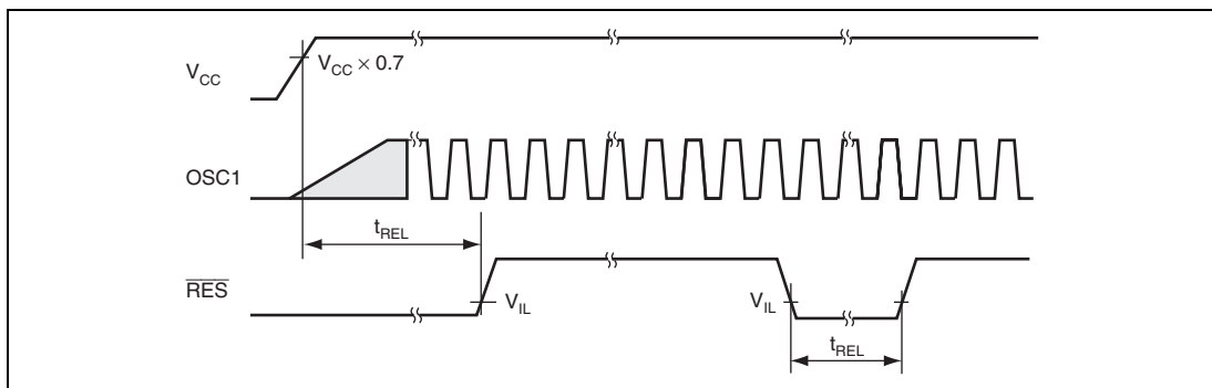
Figure 23.2 \overline{\text{RES}} Low Width Timing
