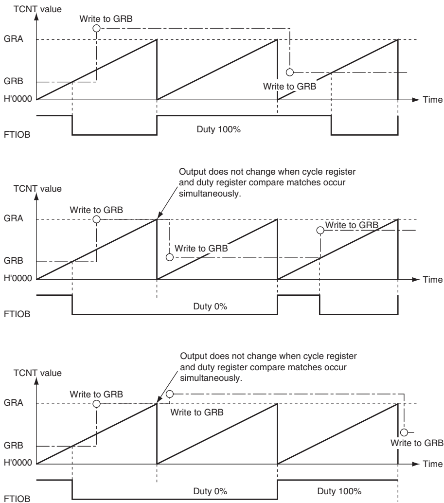
Figure 13.13 PWM Mode Example (TOB = 1, TOC = 1, and TOD = 1: Initial Output Values are Set to 1)
