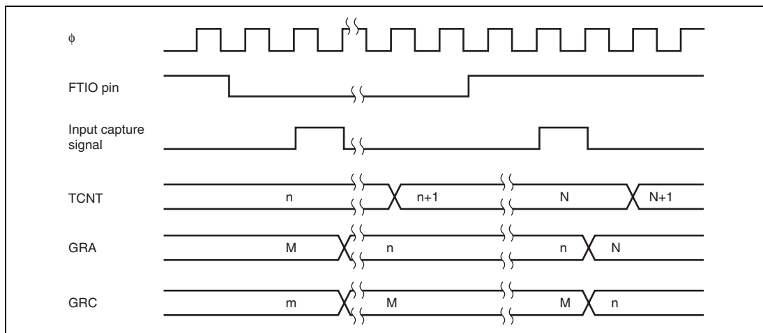
Figure 14.41 Input Capture Timing of Buffer Operation
