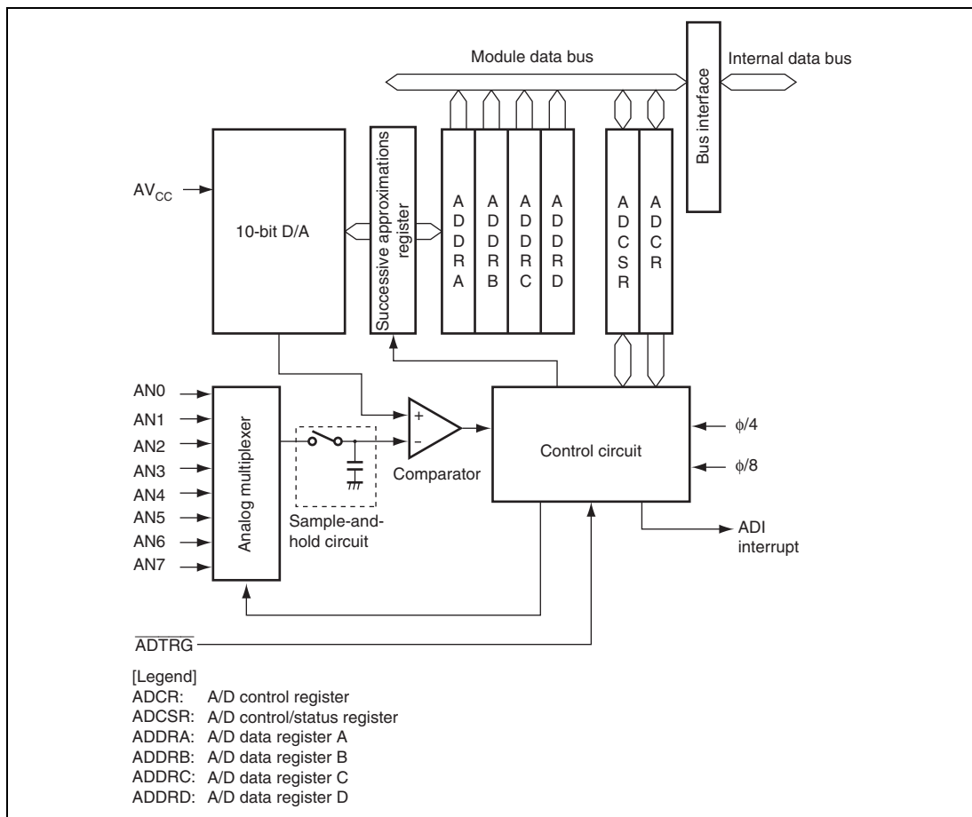
Figure 19.1 Block Diagram of A/D Converter
