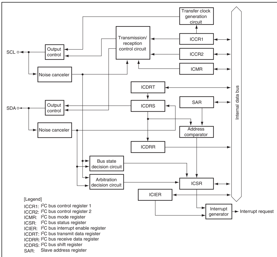
Figure 18.1 Block Diagram of I 2 C Bus Interface 2
