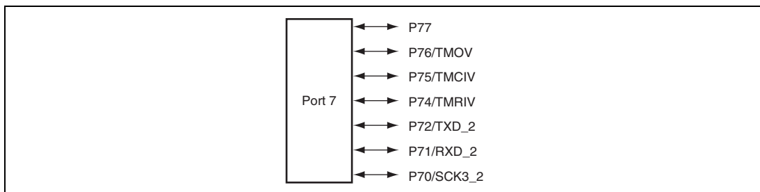
Figure 9.6 Port 7 Pin Configuration
