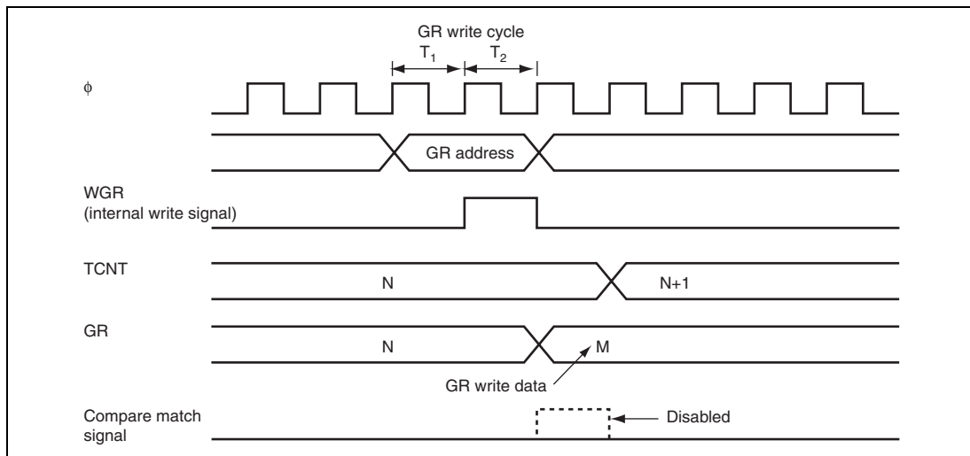
Figure 14.54 Contention between GR Write and Compare Match
