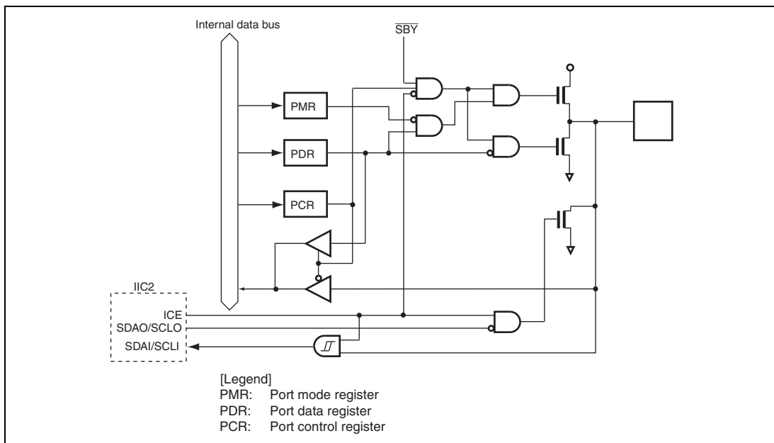
Figure B.12 Port 5 Block Diagram (P57, P56)
