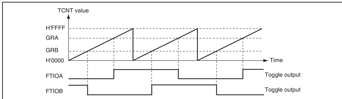
Figure 13.5 Toggle Output Example (TOA = 0, TOB = 1)
