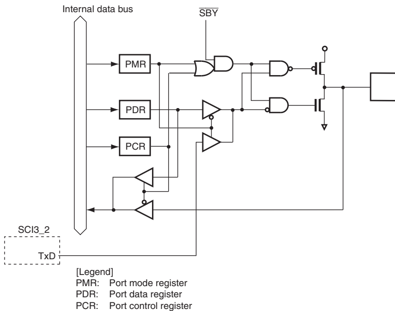
Figure B.20 Port 7 Block Diagram (P72)
