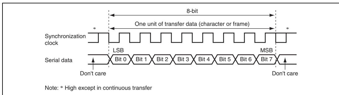
Figure 17.9 Data Format in Clocked Synchronous Communication
