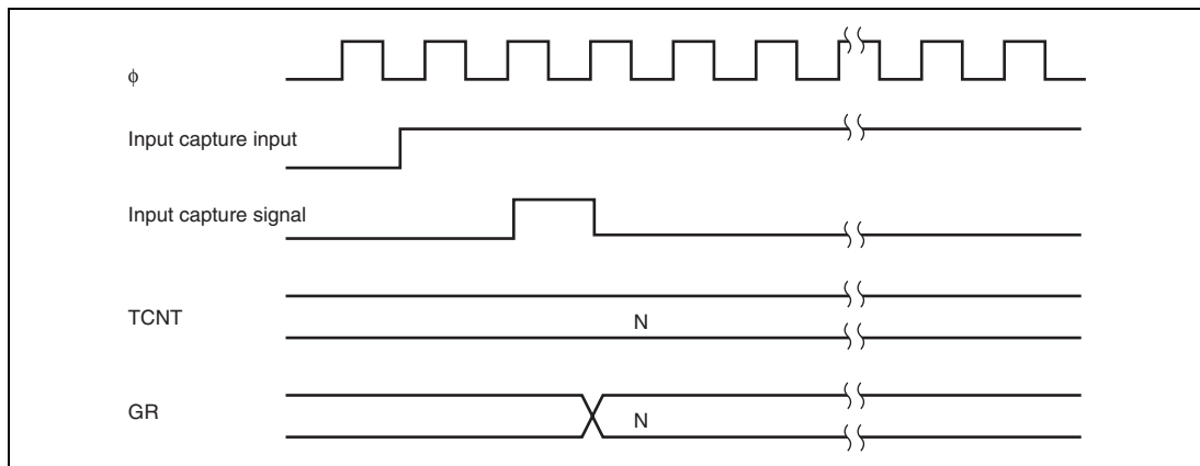
Figure 14.18 Input Capture Signal Timing
