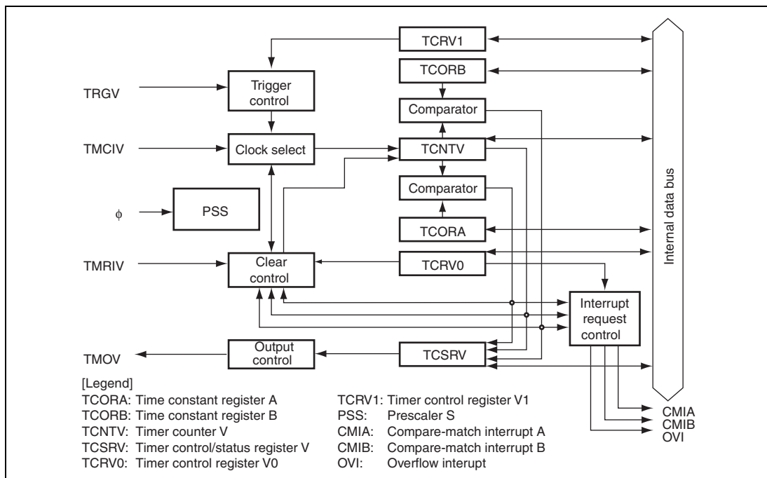
Figure 12.1 Block Diagram of Timer V
