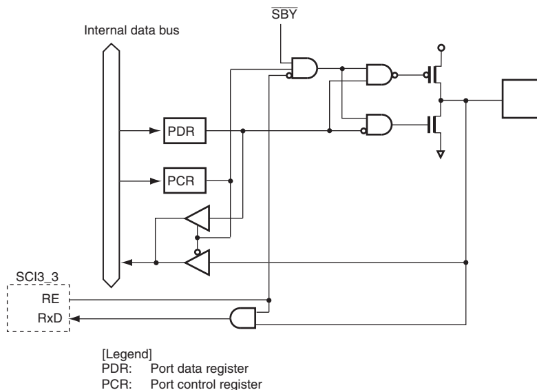
Figure B.28 Port 9 Block Diagram (P91)
