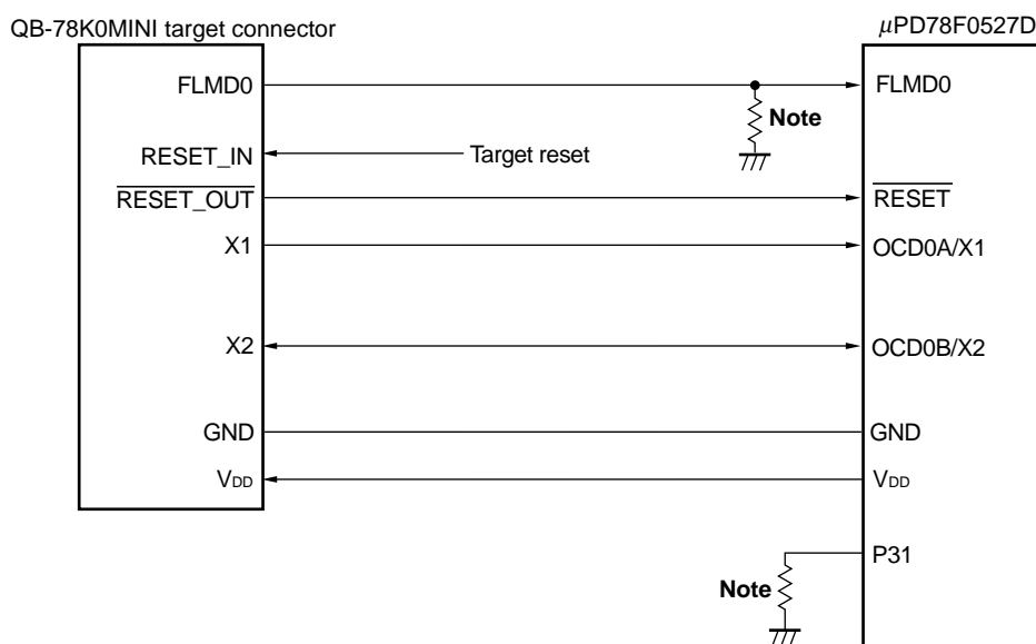
Figure 27-1. Connection Example of QB-78K0MINI and \mu PD78F0527D (When OCD0A/X1 and OCD0B/X2 Are Used)
