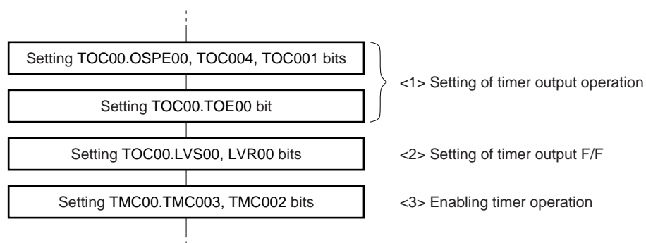
Figure 7-53. Example of Flow for Setting LVS00 and LVR00 Bits
