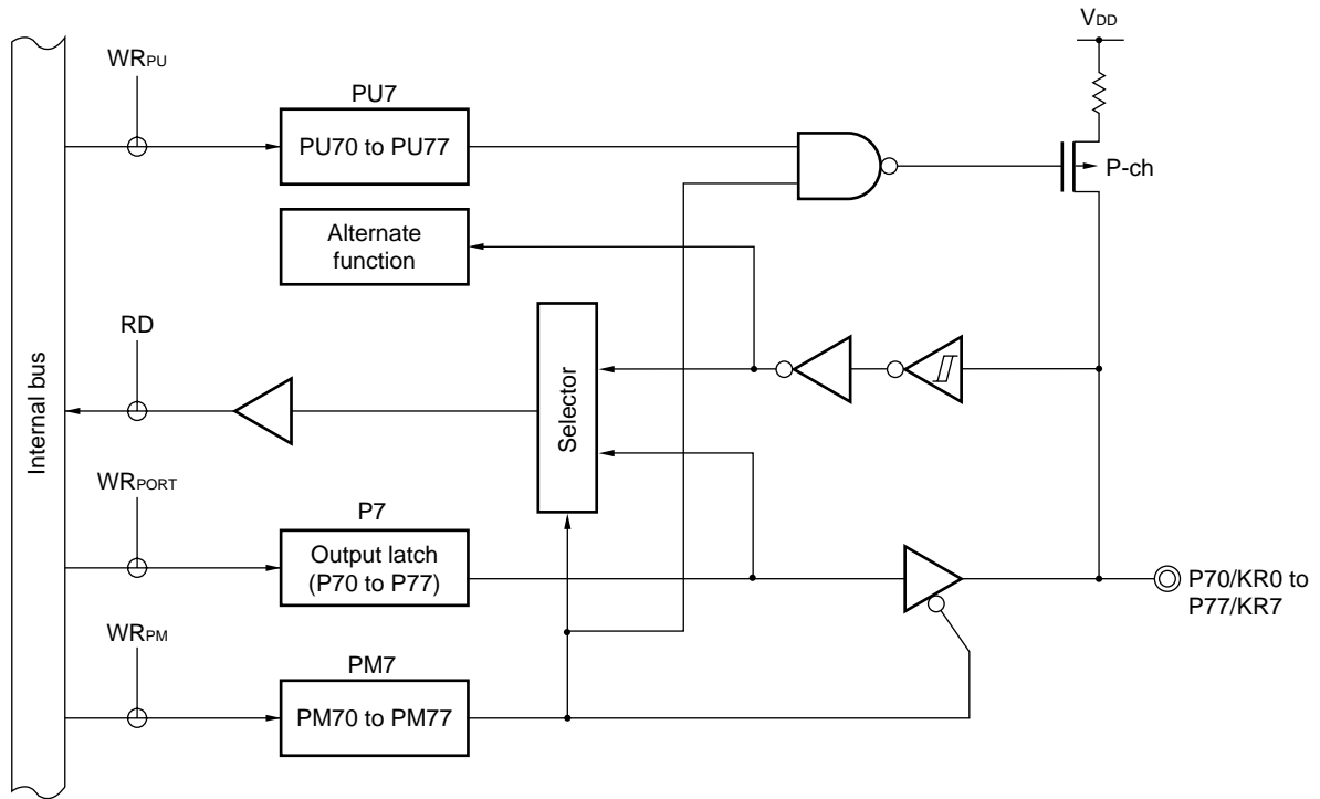
Figure 5-17. Block Diagram of P70 to P77
