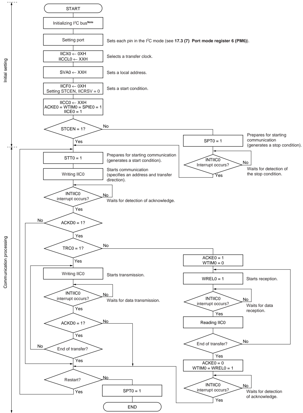
Figure 17-23. Master Operation Flowchart (Single-Master System)
