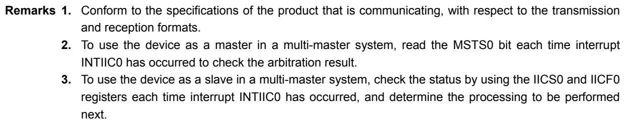
Preliminary User's Manual U17312EJ2V1UD
