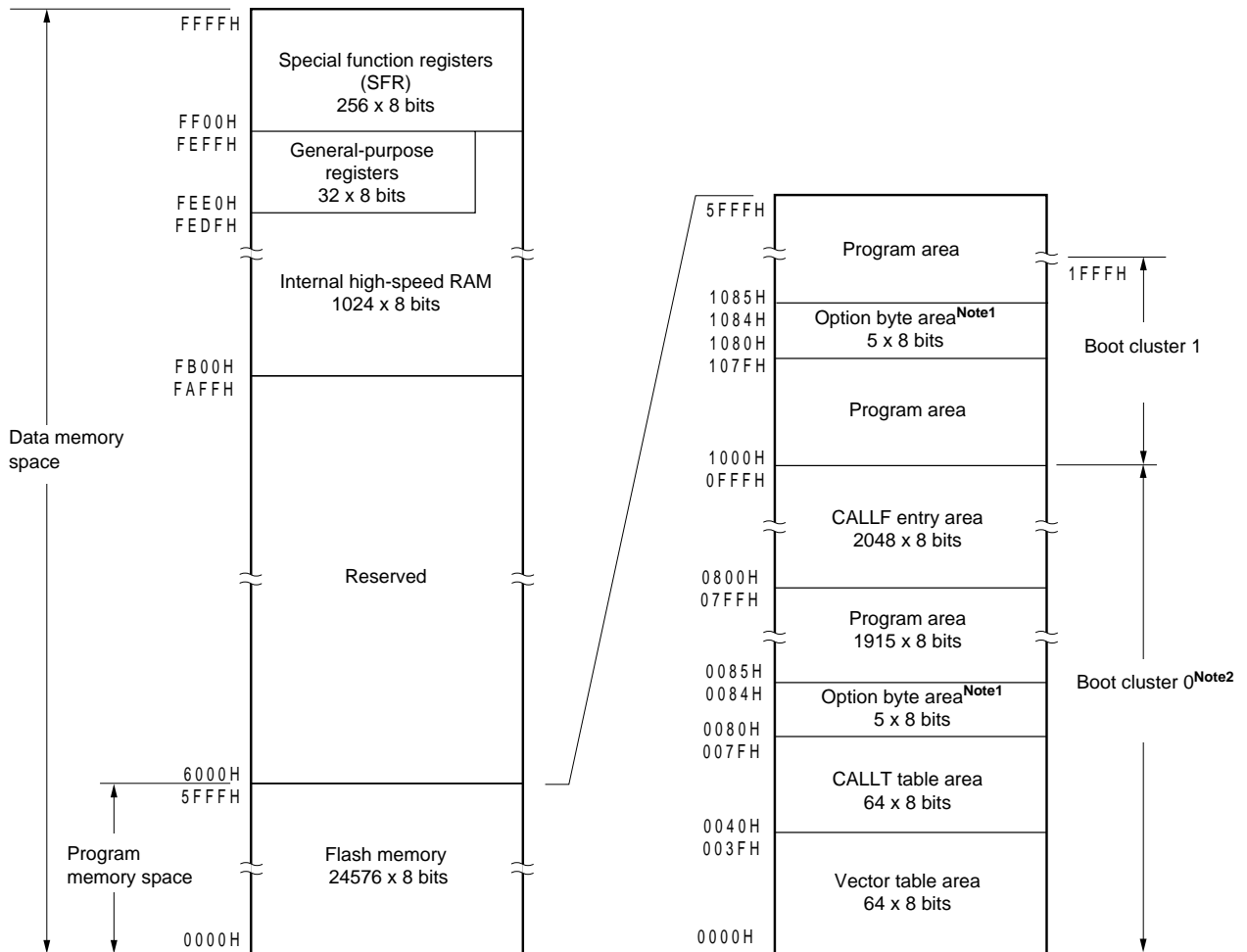
Figure 3-2. Memory Map (μPD78F0522)
