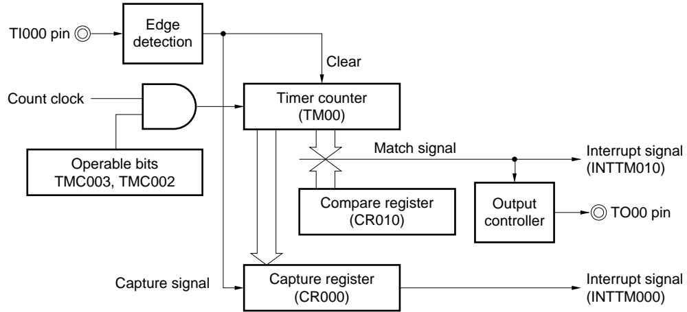
Figure 7-26. Block Diagram of Clear & Start Mode Entered by TI000 Pin Valid Edge Input (CR000: Capture Register, CR010: Compare Register)
