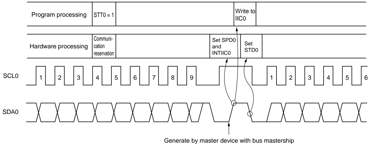
Figure 17-20. Communication Reservation Timing
