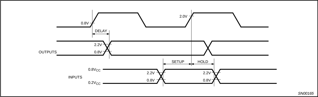
Figure 3. PR31500 Timing – Definition of AC Specification
