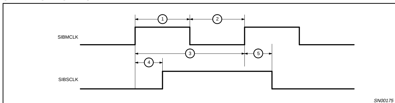
Figure 8. SIB CLK Timing
