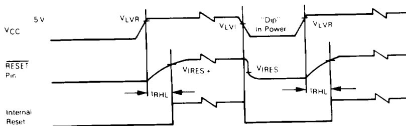
Figure 13. Power and Reset Timing
