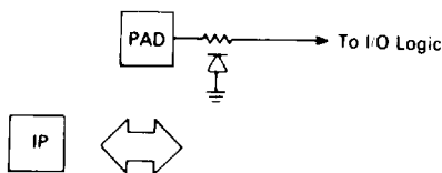
Figure 16. Typical Input Protection
