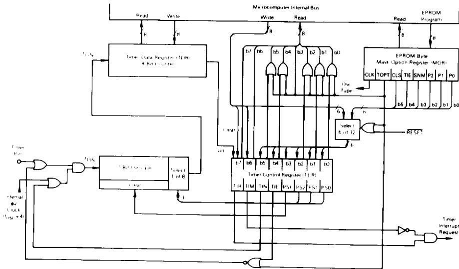
Figure 9. Timer Block Diagram
