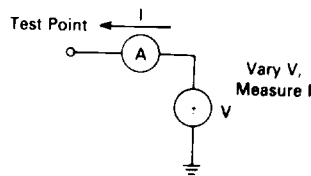
Figure 17. I/O Characteristic Measurement Circuit
