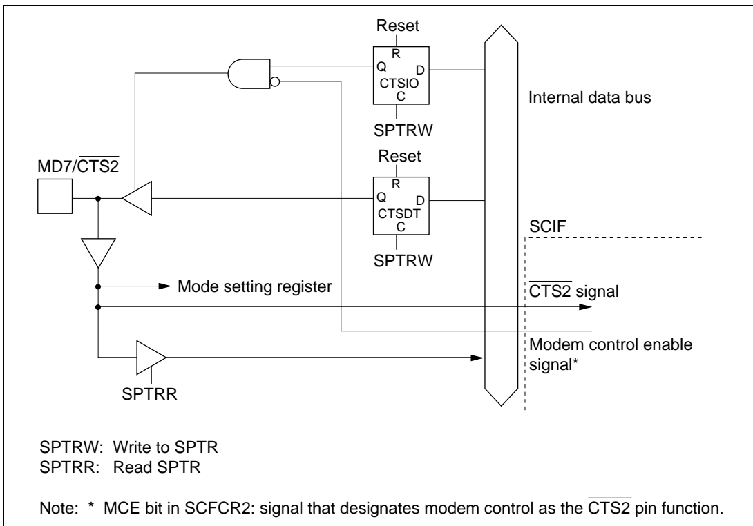
Figure 18.9 MD7/CTS2 Pin
