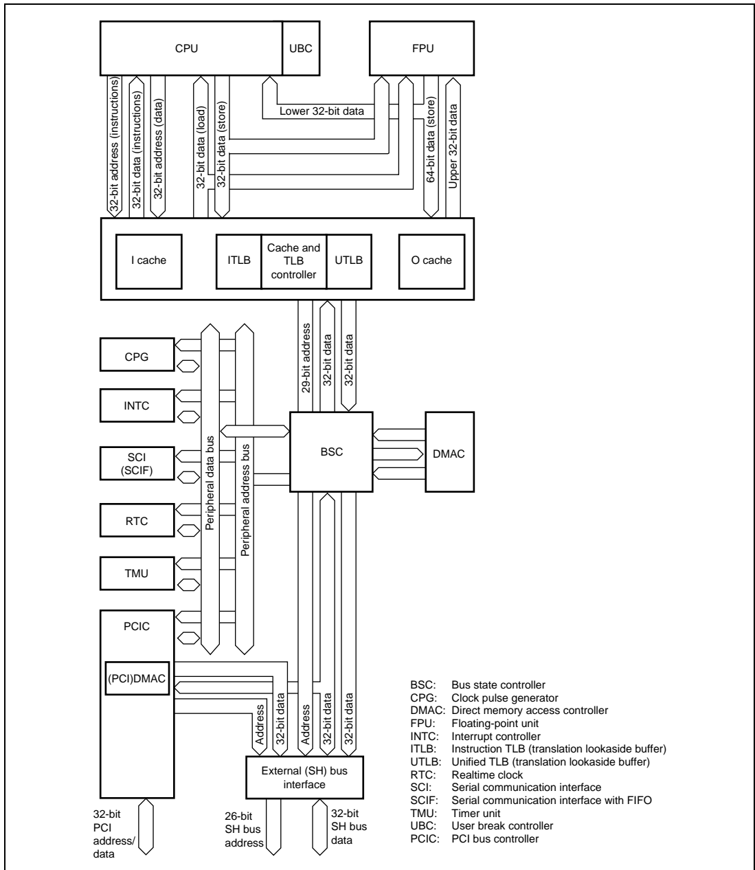
Figure 1.1 Block Diagram of SH7751 Series Functions
