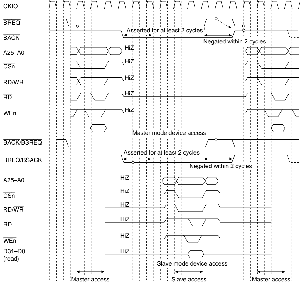
Figure 13.73 Arbitration Sequence
