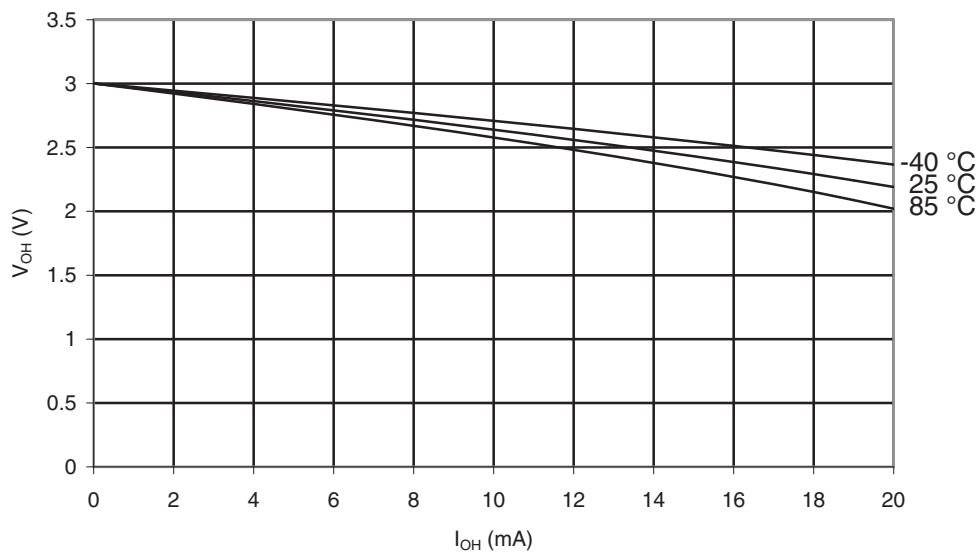
Figure 29-369. ATmega1284P: I/O Pin Output Voltage vs. Source Current ( V_{CC} = 3V )
