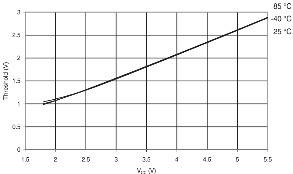
Figure 29-172. ATmega324PA: I/O Pin Input Threshold vs. V_{CC} ( V_{IH} , I/O Pin Read as '1').
