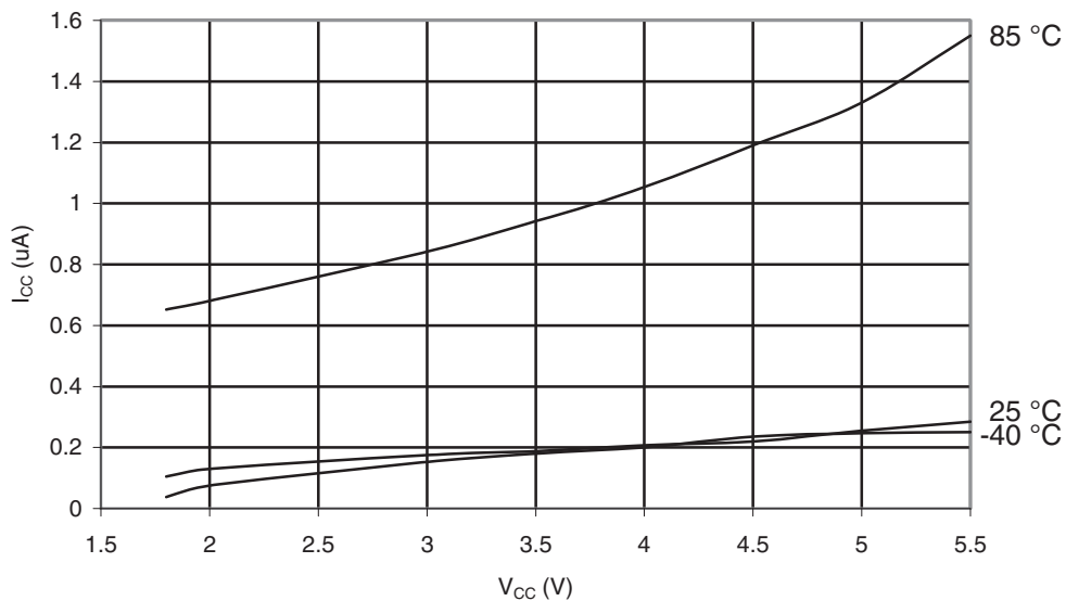
Figure 29-11. ATmega164A: Power-down Supply Current vs. V_{CC} (Watchdog Timer Disabled).
