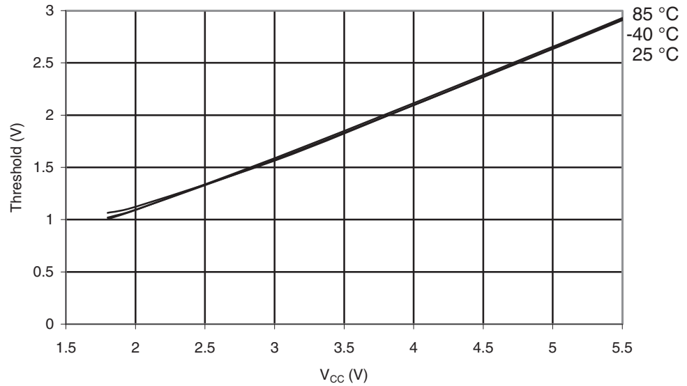
Figure 29-222. ATmega644A: I/O Pin Input Threshold vs. V_{CC} ( V_{IL} , I/O Pin Read as '0').
