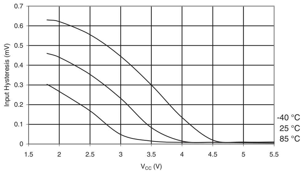
Figure 29-30. ATmega164A: Reset Pin Input Hysteresis vs. V_{CC}
