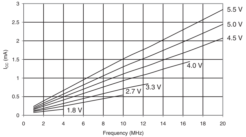
Figure 29-301. ATmega1284: Idle Supply Current vs. Frequency (1 - 20MHz)
