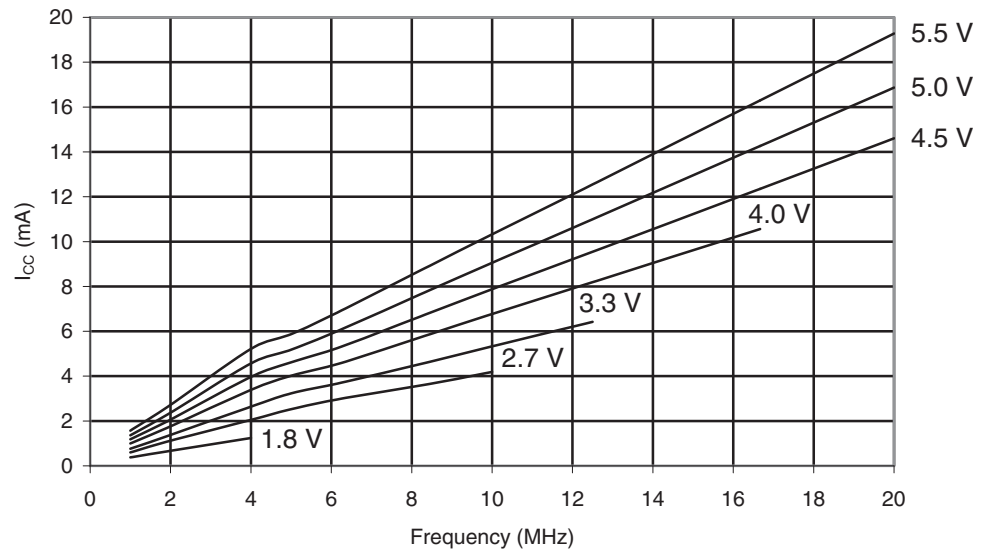
Figure 29-346. ATmega1284P: Active Supply Current vs. Frequency (1 - 20MHz)
