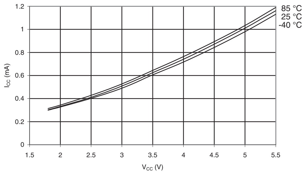
Figure 29-4. ATmega164A: Active Supply Current vs. V_{CC} (Internal RC Oscillator, 1MHz).
