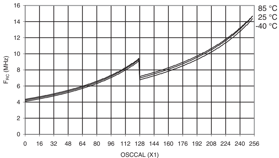
Figure 29-335. ATmega1284: Calibrated 8MHz RC Oscillator vs. OSCCAL Value
