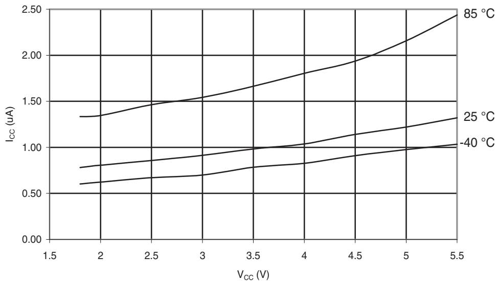
Figure 29-160. ATmega324PA: Power-save Supply Current vs. V_{CC} (Watchdog Timer Disabled and 32kHz Crystal Oscillator Running).
