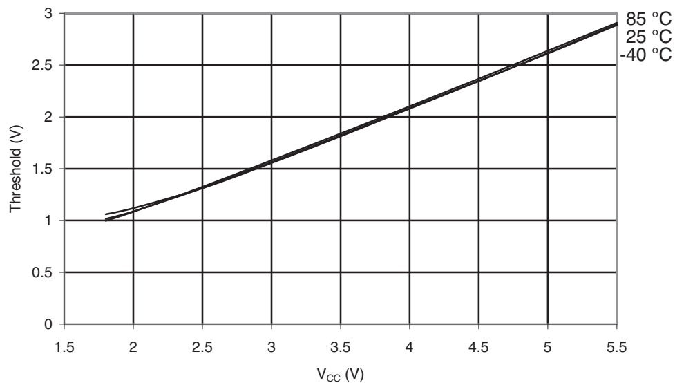
Figure 29-370. ATmega1284P: I/O Pin Input Threshold vs. V_{CC} ( V_{IH} , I/O Pin Read as '1')
