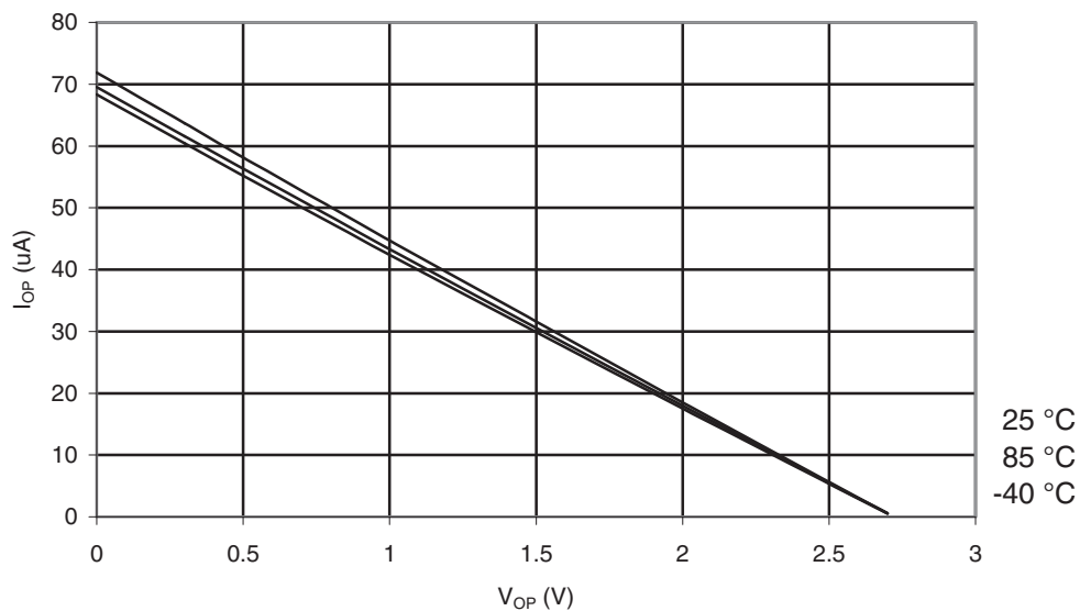
Figure 29-65. ATmega164PA: I/O Pin Pull-up Resistor Current vs. Input Voltage ( V_{CC} = 2.7V ).
