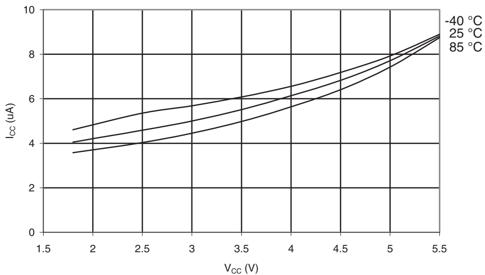
Figure 29-12. ATmega164A: Power-down Supply Current vs. V_{CC} (Watchdog Timer Enabled).
