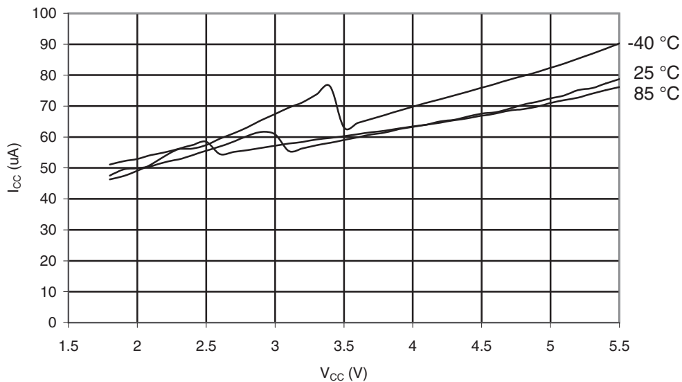
Figure 29-42. ATmega164A: Analog Comparator Current vs. V_{CC}
