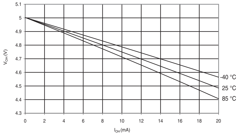
Figure 29-220. ATmega644A: I/O Pin Output Voltage vs. Source Current ( V_{CC} = 5V )
