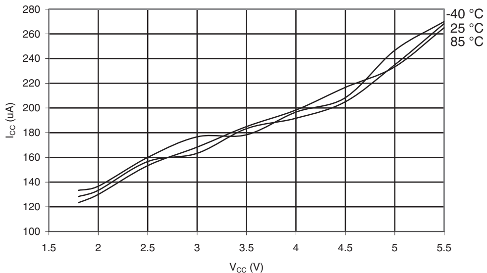
Figure 29-336. ATmega1284: ADC Current vs. V_{CC} (AREF = AV_{CC} )
