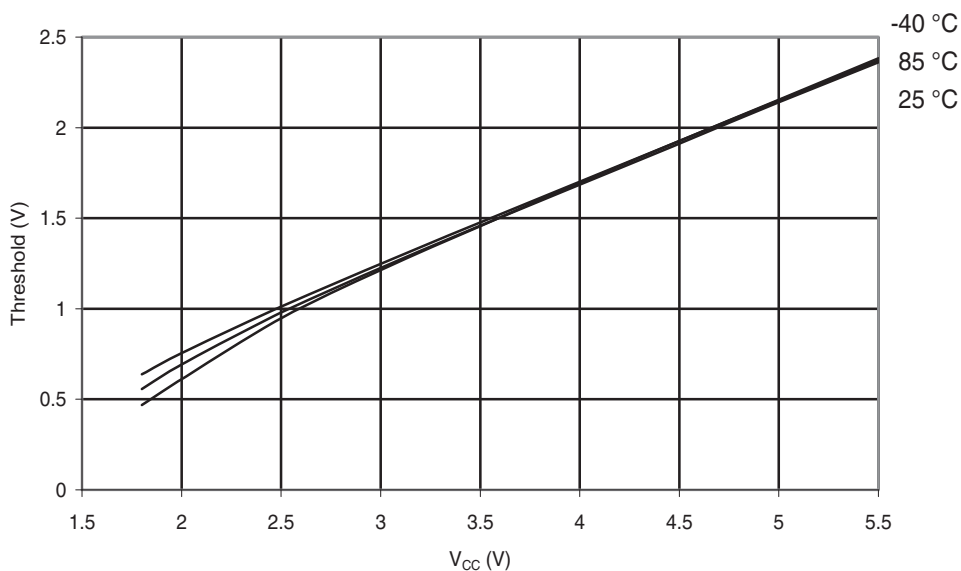
Figure 29-173. ATmega324PA: I/O Pin Input Threshold vs. V_{CC} ( V_{IL} , I/O Pin Read as '0').
