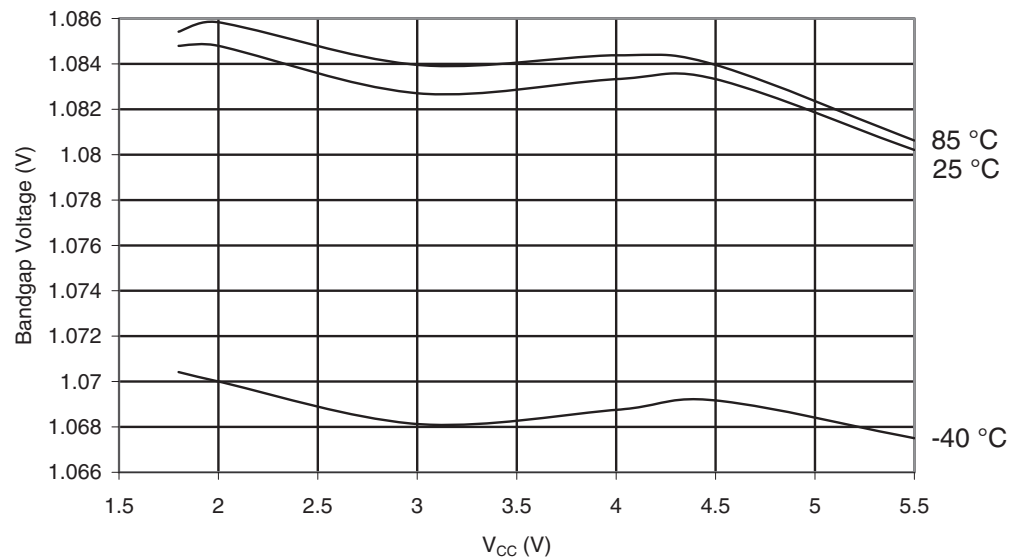
Figure 29-279. ATmega644PA: Calibrated Bandgap Voltage vs. V_{CC}
