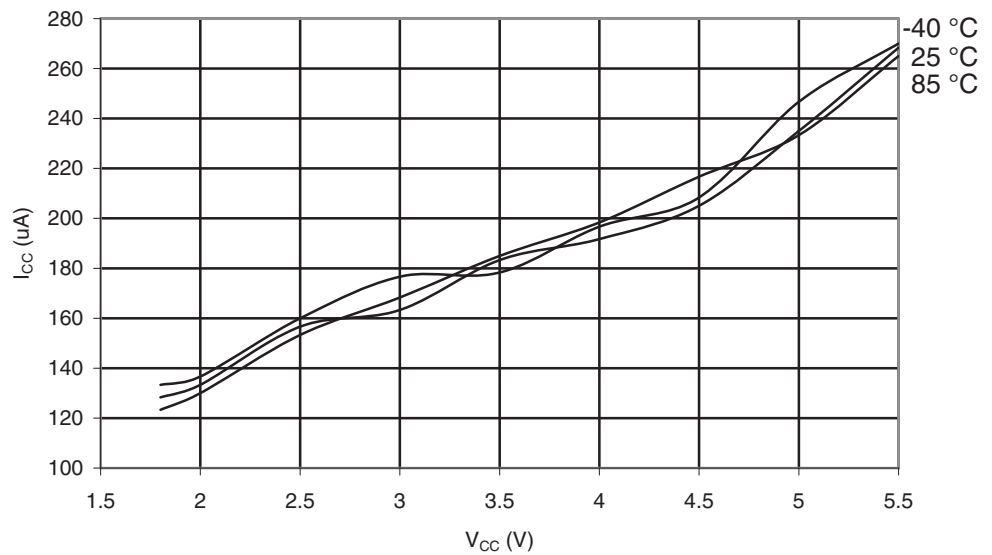
Figure 29-386. ATmega1284P: ADC Current vs. V_{CC} (AREF = AV_{CC} )
