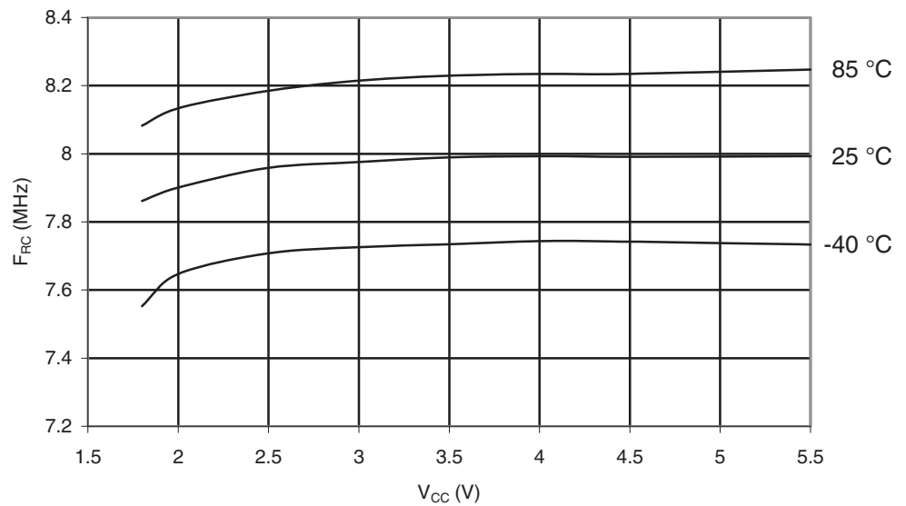
Figure 29-87. ATmega164PA: Calibrated 8MHz RC Oscillator vs. V_{CC}
