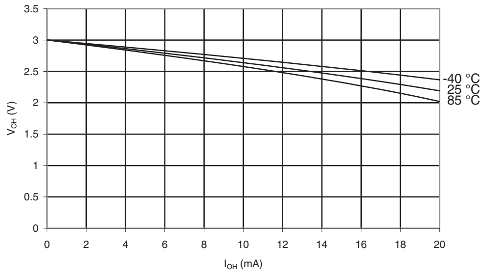
Figure 29-319. ATmega1284: I/O Pin Output Voltage vs. Source Current ( V_{CC} = 3V )
