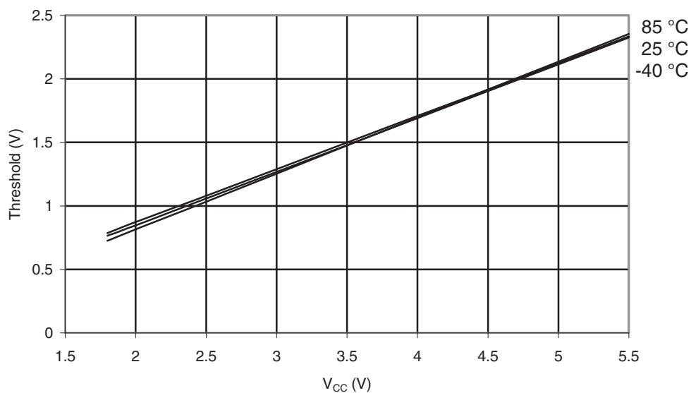
Figure 29-29. ATmega164A: Reset Pin Input Threshold vs. V_{CC} ( V_{IL} , I/O Pin Read as '0').
