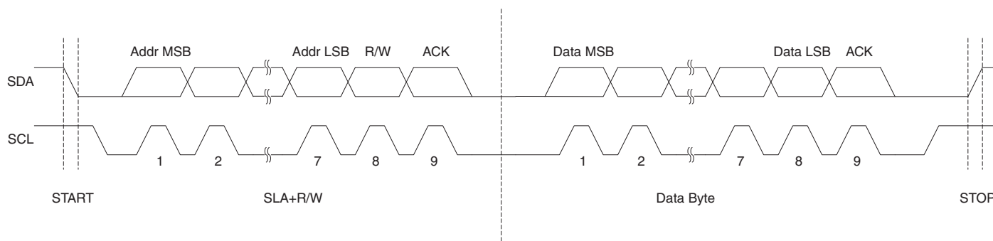
Figure 21-6. Typical Data Transmission
