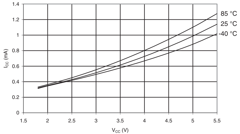
Figure 29-302. ATmega1284: Idle Supply Current vs. V_{CC} (Internal RC Oscillator, 8MHz)
