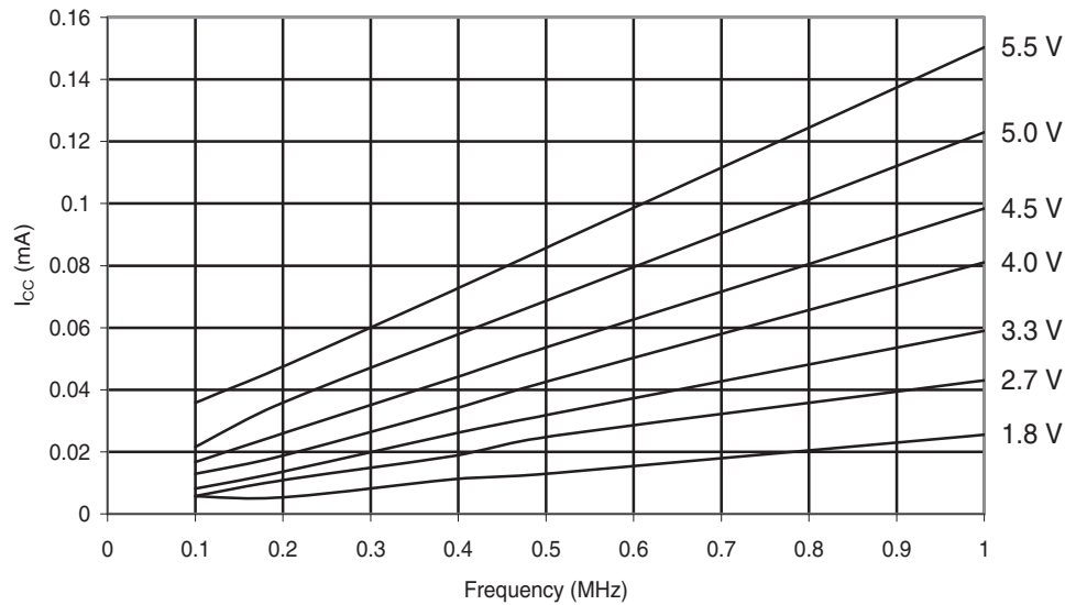
Figure 30-6. ATmega48A: Idle Supply Current vs. Low Frequency (0.1-1.0MHz)
