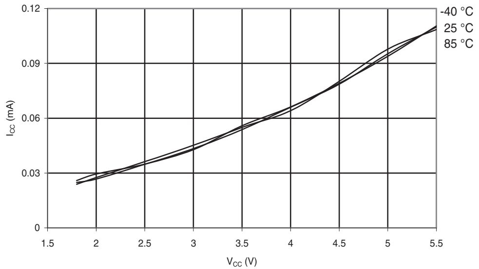
Figure 30-97. ATmega88A: Active Supply Current vs. V_{CC} (Internal RC Oscillator, 128kHz)
