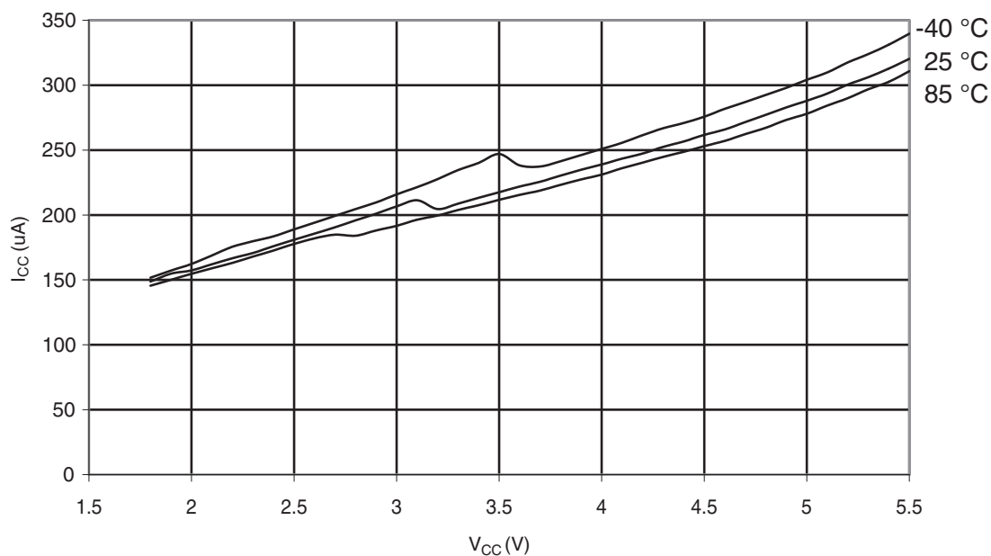
Figure 30-322. ATmega328: ADC Current vs. V_{CC} (AREF = AV_{CC} )
