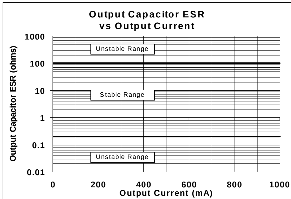
Figure 19. Output Cap ESR vs. I_{out} .
