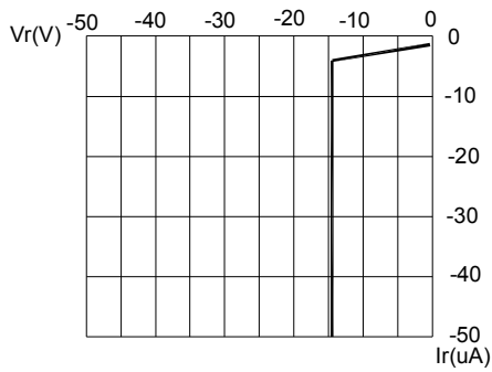
FIG.3 Green & Blue REVERSE CURRENT VS. REVERSE VOLTAGE.
