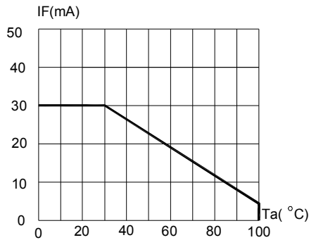
FIG.5 RED & YELLOW MAXIMUM FORWARD DC CURRENT VS AMBIENT TEMPERATURE ( T_{jmax}=105^{\circ}C )
