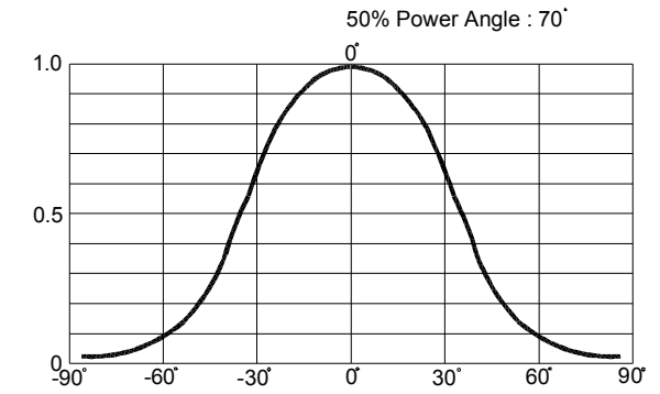
FIG.6 RED & BLUE&GREEN FAR FIELD PATTERN
