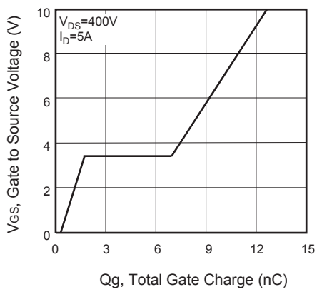
Figure 7. Gate Charge
