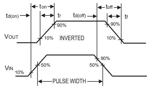
Figure 10. Switching Waveforms
