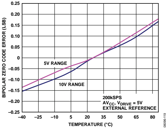
Figure 21. Bipolar Zero Code Error vs. Temperature
