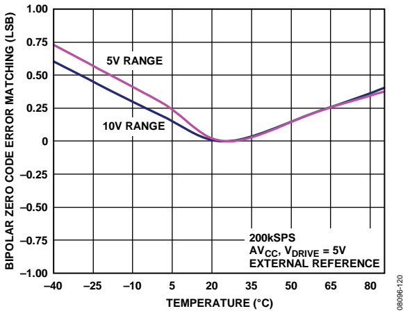
Figure 22. Bipolar Zero Code Error Matching vs. Temperature
