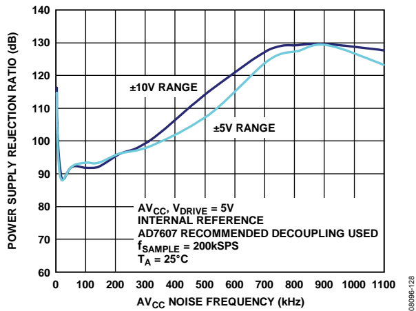
Figure 28. PSRR
