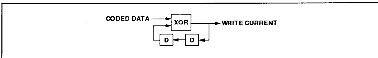
FIGURE 12: Precoder Block Diagram
