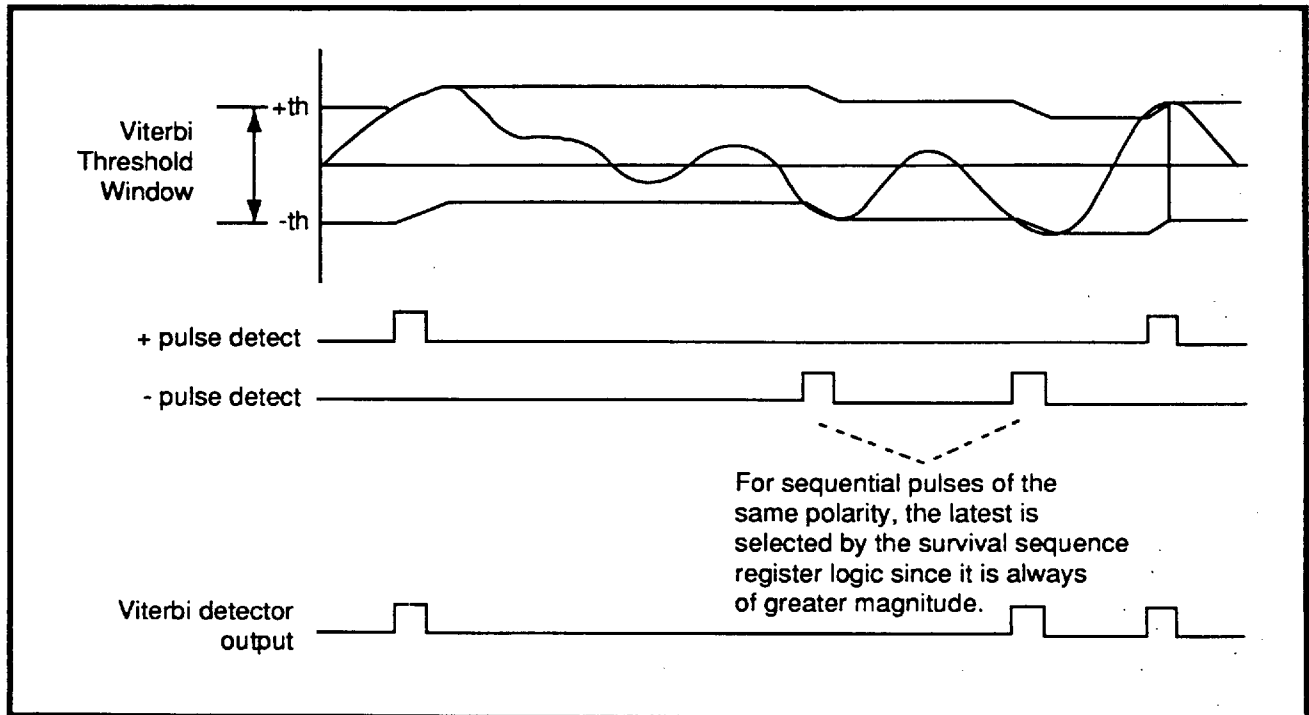
FIGURE 4: Viterbi Detection
