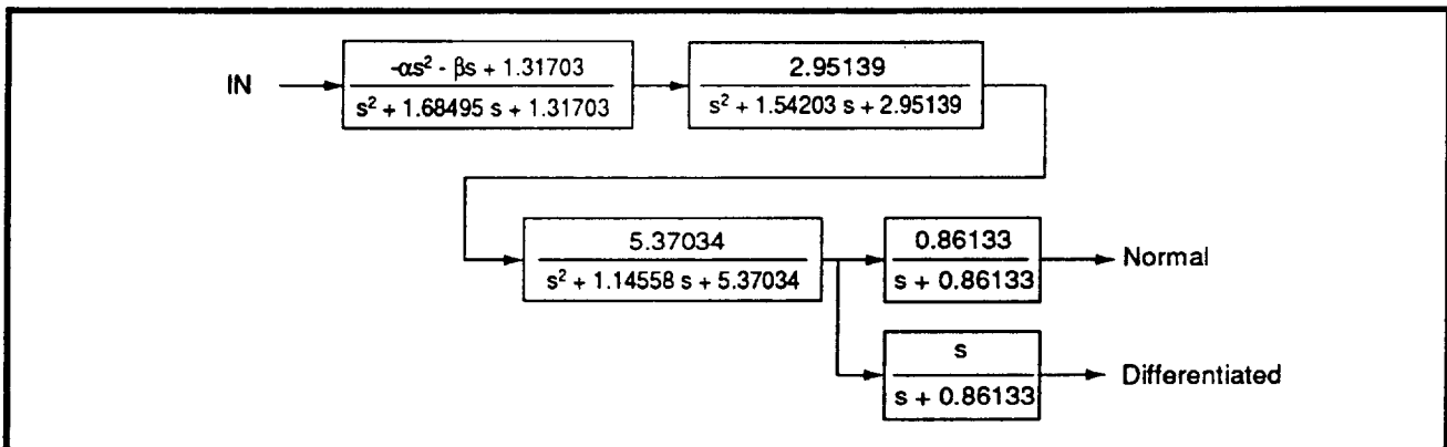
FIGURE 5: Programmable Filter Normalized Transfer Function
