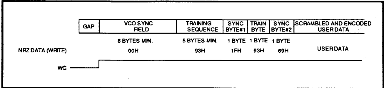
FIGURE 17: Hard Sector Write Sequence - Dual Sync
