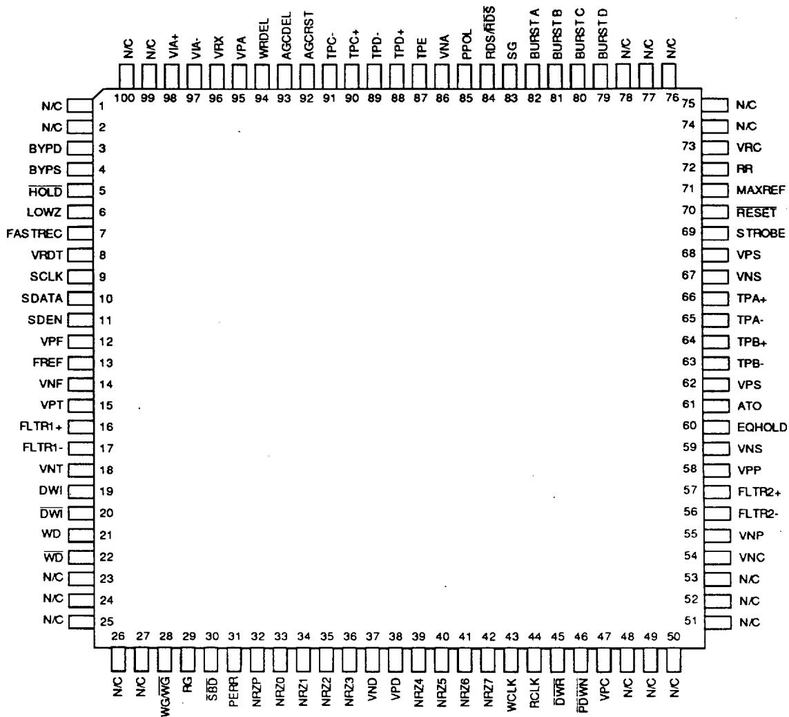
100-Lead TQFP
