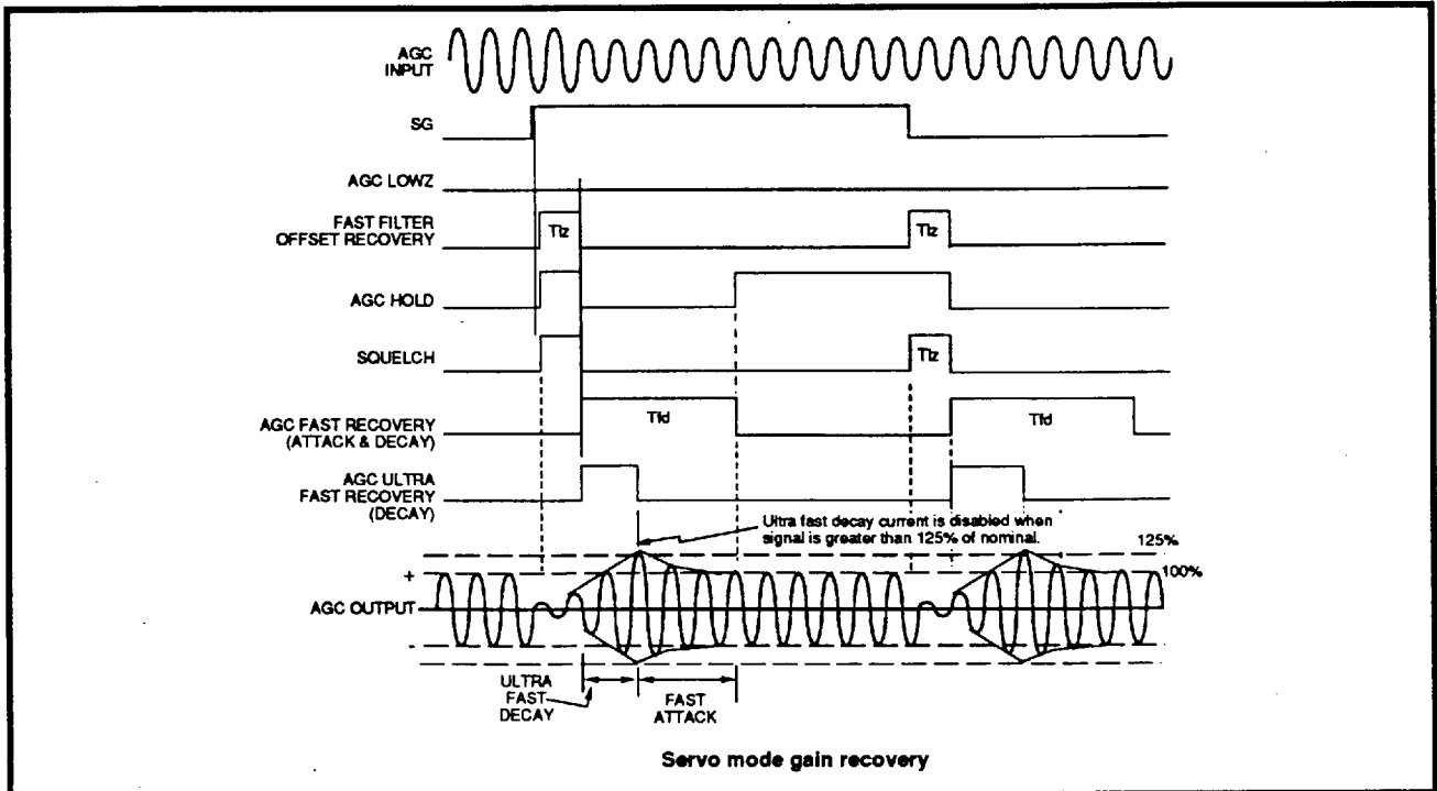
FIGURE 2: AGC Timing Diagrams - Servo Mode
