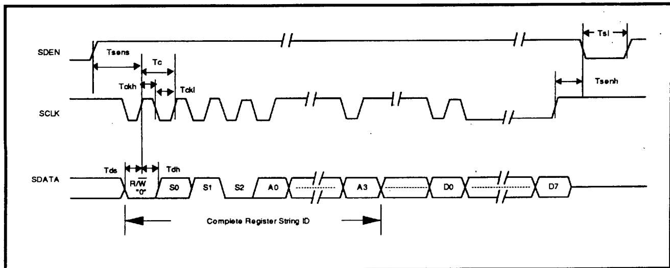
FIGURE 16: Serial Interface Timing
