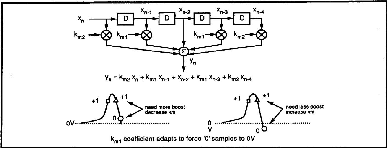
FIGURE 8: Block Diagram of 5-Tap Equalizer
