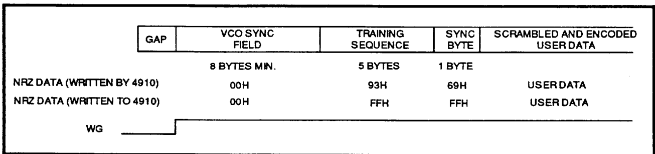
FIGURE 18: Hard Sector Semi-Auto Write Mode
