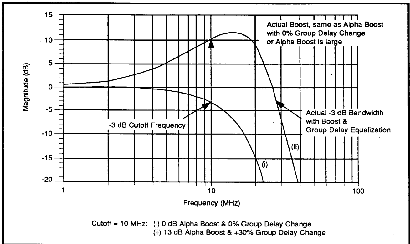
FIGURE 6: Filter Magnitude Response
