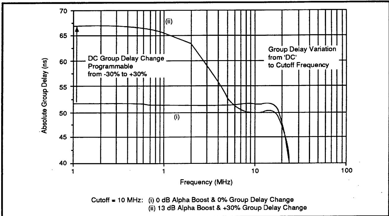
FIGURE 7: Filter Group Delay Response
