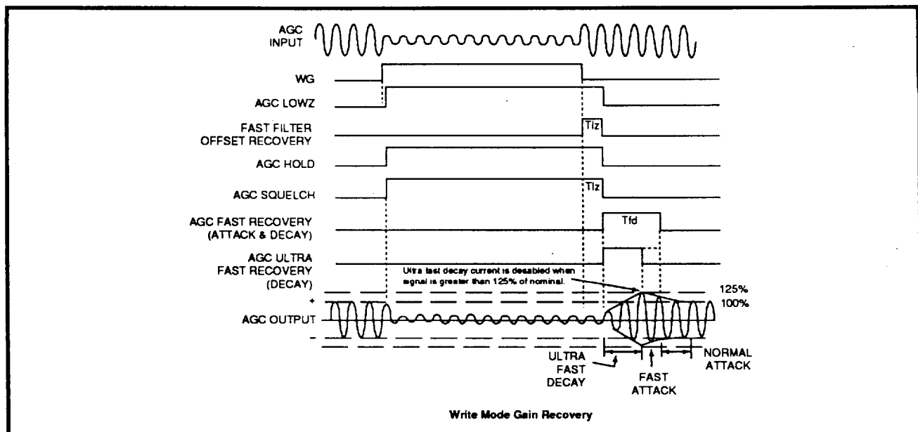
FIGURE 3: AGC Timing Diagrams - Write Mode
