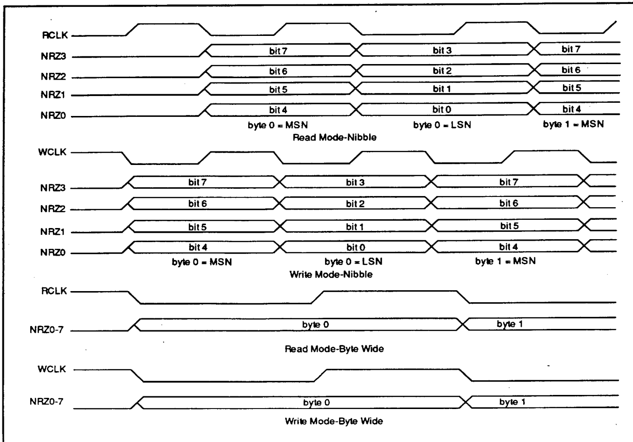
FIGURE 11: NRZ Timing
