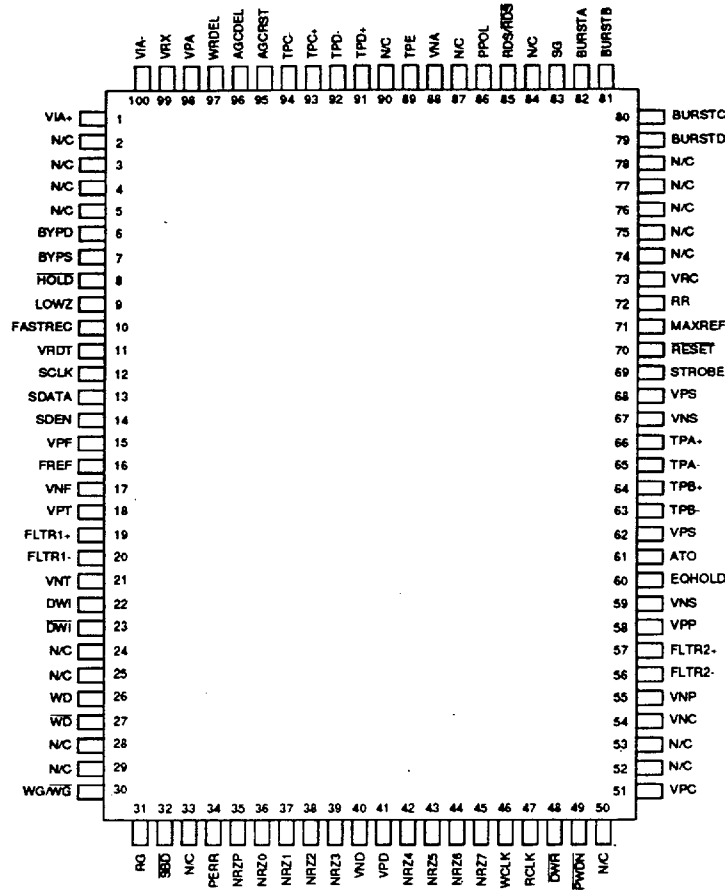
100-Lead QFP
