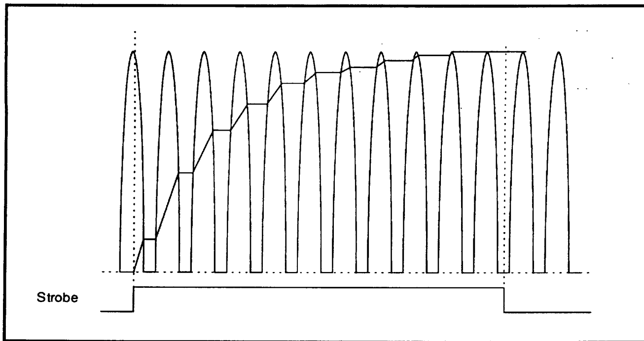
FIGURE 14: Servo Burst Acquisition (SG= \overline{\text{RESET}} = 1)
