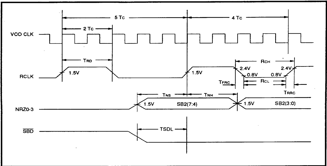
FIGURE 24: Nibble Read Timing
