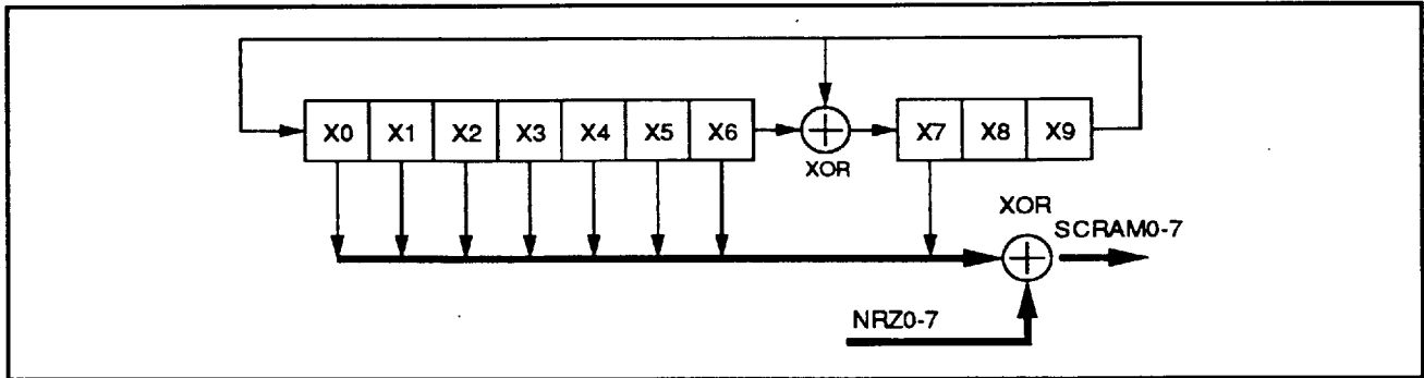
FIGURE 10: Scrambler Block Diagram
