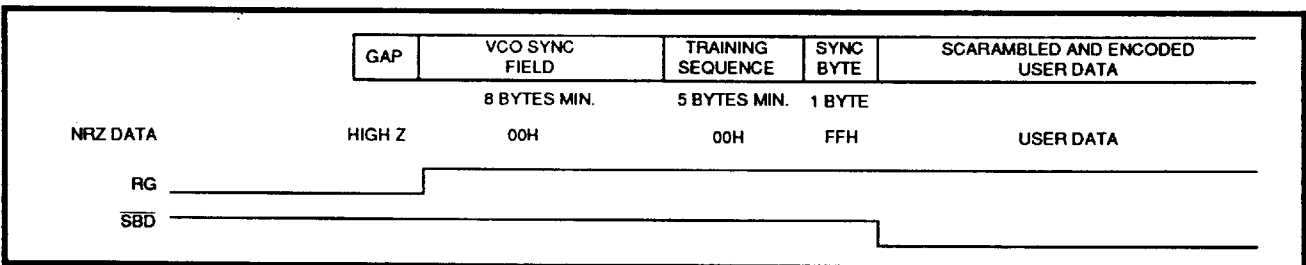
FIGURE 20: Semi-Auto Sector Read Mode
