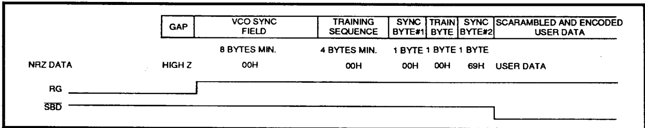
FIGURE 19: Read Sequence - Dual Sync Byte Mode
