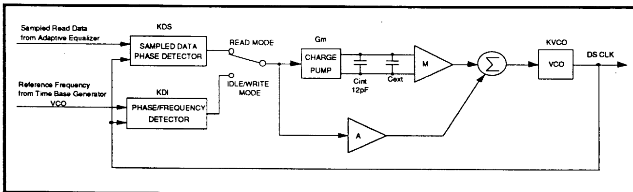
FIGURE 9: Data Synchronizer Phase Locked Loop
