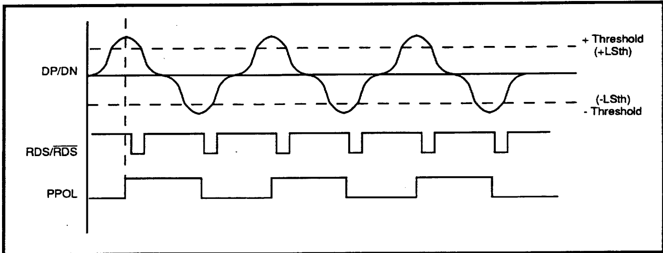
FIGURE 15: RDS/RDS and PPOL vs. DP/DN Relationship
