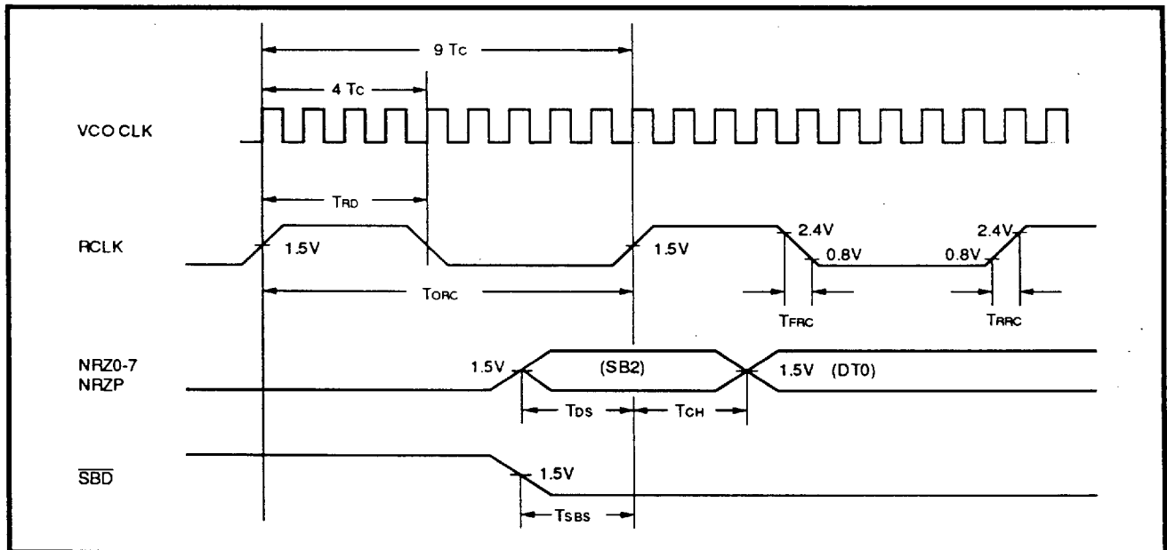
FIGURE 22: Byte Wide Read Timing
