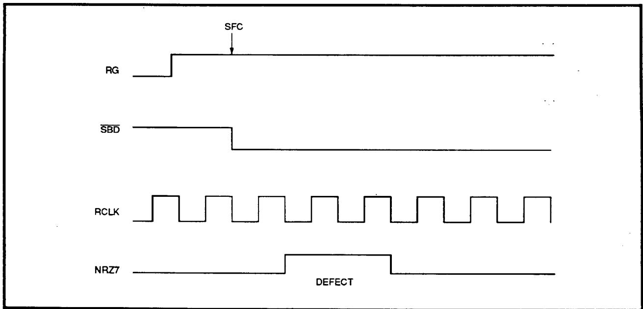
FIGURE 21: Surface Defect Scan Mode
