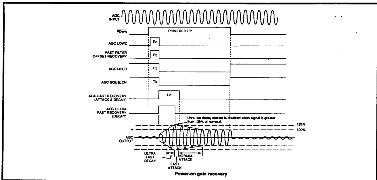
FIGURE 1: AGC Timing (Internal) Diagrams - Power-On Mode
