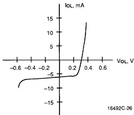
Output, LOW
