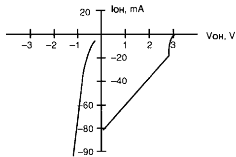
Output, HIGH
