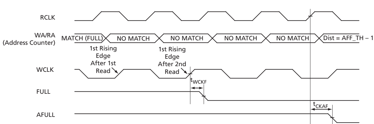
Figure 2-56 • FIFO FULL Flag and AFULL Flag Deassertion
