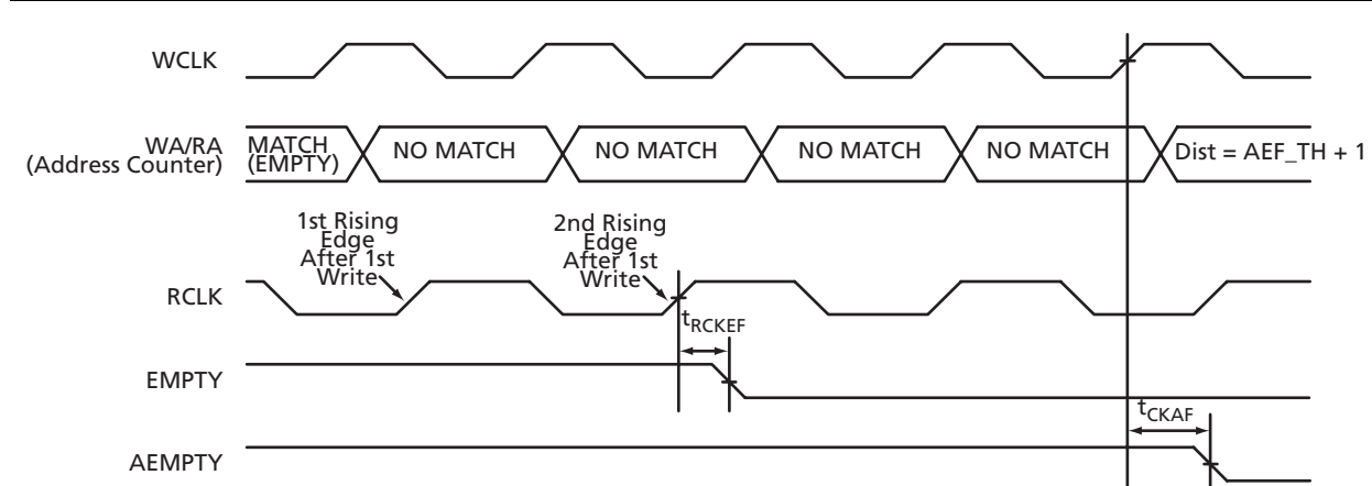
Figure 2-55 • FIFO EMPTY Flag and AEMPTY Flag Deassertion
