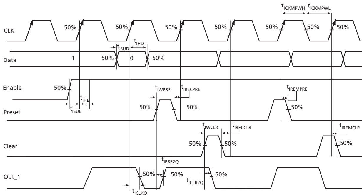
Figure 2-29 • Input Register Timing Diagram
