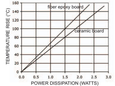
POWER DERATING
