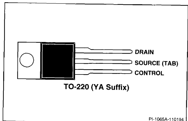
Figure 3. Pin Configuration.
