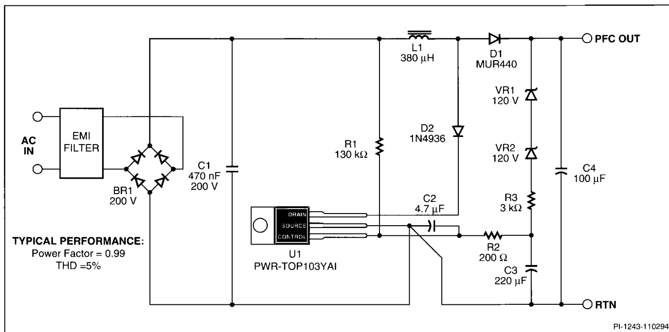
Figure 10. Schematic Diagram of a 60 W 110 VAC Input Boost Power Factor Correction Circuit Utilizing the PWR-TOP103.
