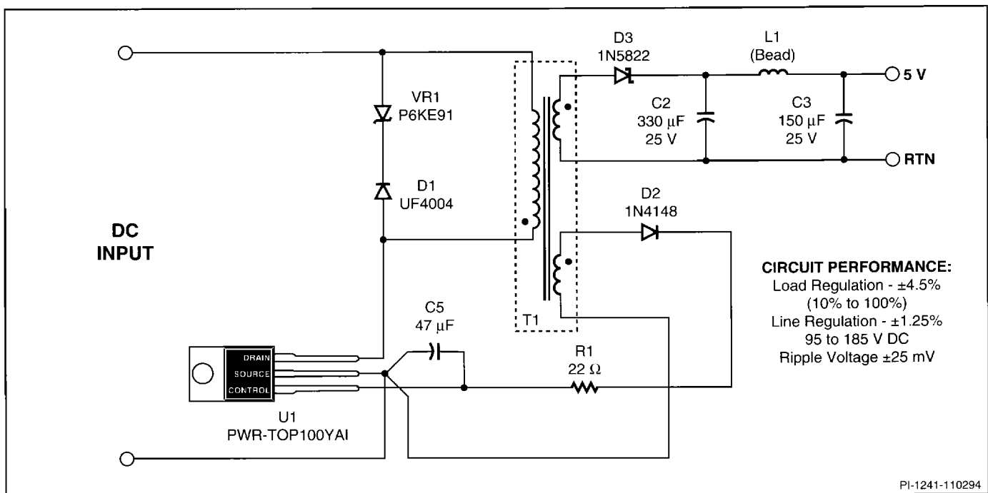
Figure 7. Schematic Diagram of a Minimum Parts Count 5 V, 5 W Bias Supply Utilizing the PWR-TOP100.
