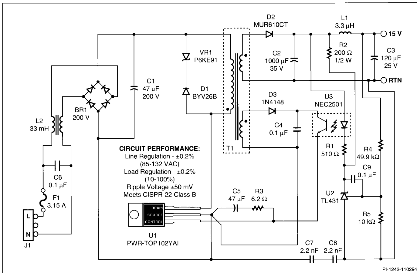
Figure 9. Schematic Diagram of a 30 W 100/110 VAC Input Power Supply Utilizing the PWR-TOP102 and Accurate Optocoupler Feedback.
