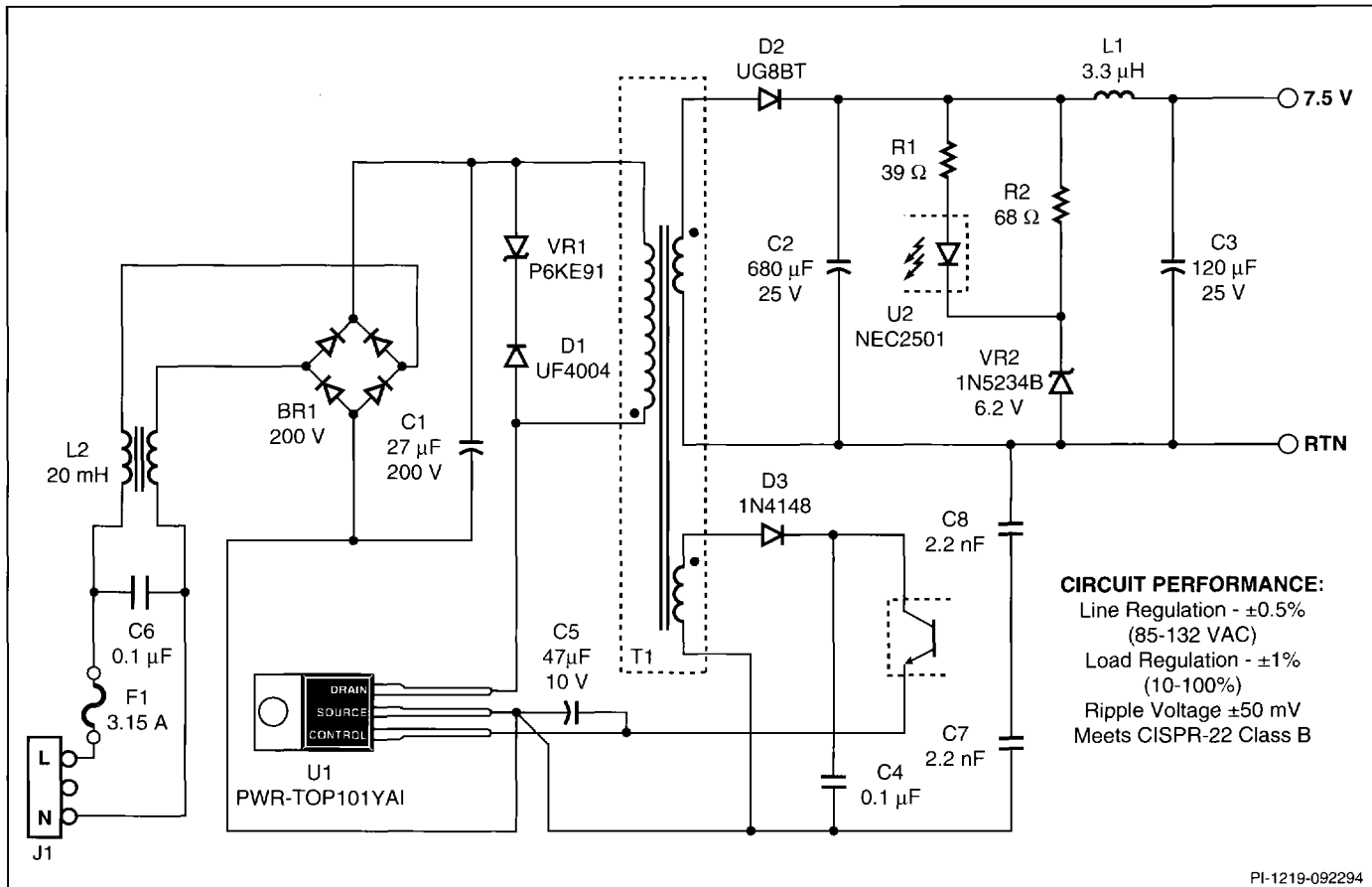
Figure 8. Schematic Diagram of a 15 W 100/110 VAC Input Power Supply Utilizing the PWR-TOP101 and Simple Optocoupler Feedback.
