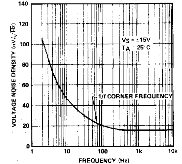
VOLTAGE NOISE DENSITY vs FREQUENCY
